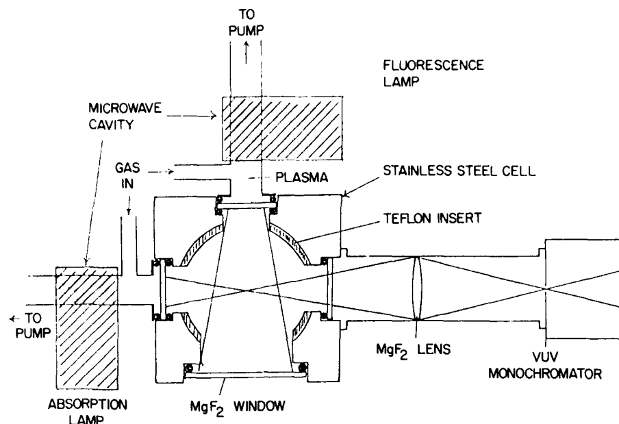
Figure 2. Cross Sectional View of the Absorption/Fluorescence Cell Showing the Placement of the Lamps. The direction of the flow in the reactor is perpendicular to the figure
