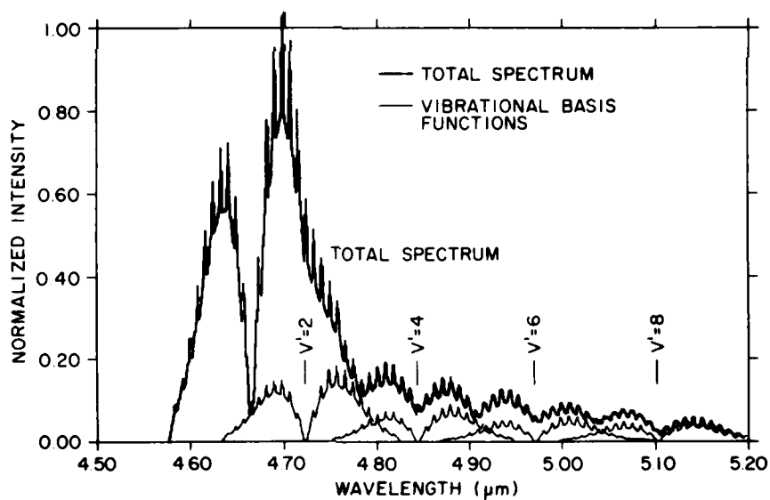
Figure 22. Computed Least Squares Spectral Fit to the Experimental CO Spectrum of Figure 21. T_{ROT} = 80K , \delta\lambda = 0.007 \mu m
