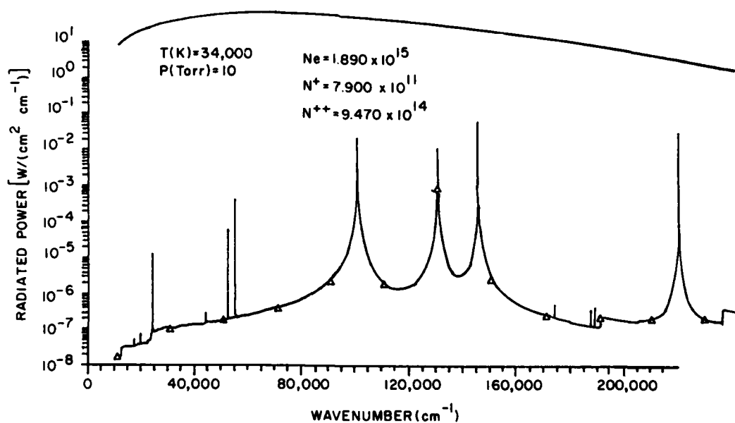
Figure 16. Emission by an Equilibrium Nitrogen Plasma Slab of Thickness 0.2 mm in the 0 to 250,000 \text{cm}^{-1} Band, T = 34,000 \text{ K} , p = 10 \text{ Torr}
