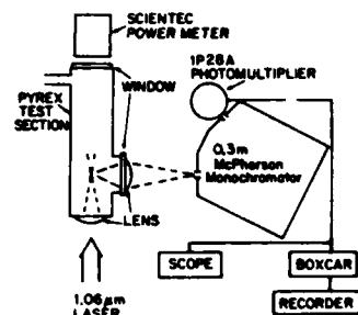
Fig. 1. Schematic diagram of the experimental apparatus. The monochromator was not used in the breakdown threshold measurements (see text).
