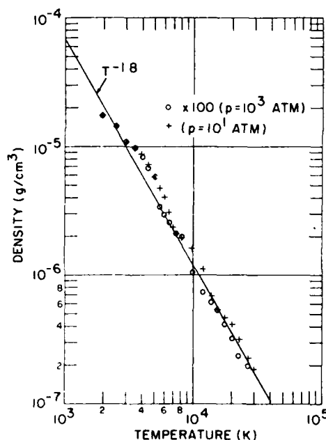
Figure 26. Density of Nitrogen
