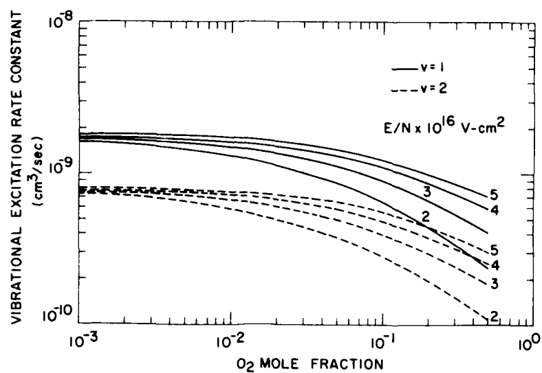
Figure 7. Predicted Rate Constants for Direct Excitation of Vibrational Levels v = 1 and 2 of \text{O}_2 in Microwave Excited Mixtures of \text{O}_2/\text{Ar}
