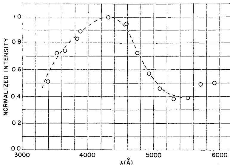
Figure 1. Continuum Spectrum Using 125 Torr \text{N}_2 and I = 9.8 \times 10^{11} \text{ W/cm}^2
