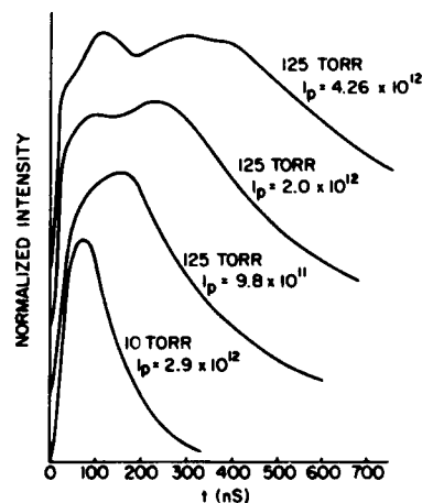
Fig. 5. Temporal profile of the 444.7-nm line of N ^+ . I_p is peak laser intensity in W cm ^{-2} at the pressures indicated. The 10-Torr and first 125-Torr curves are generated at I_p of twice threshold for breakdown.
