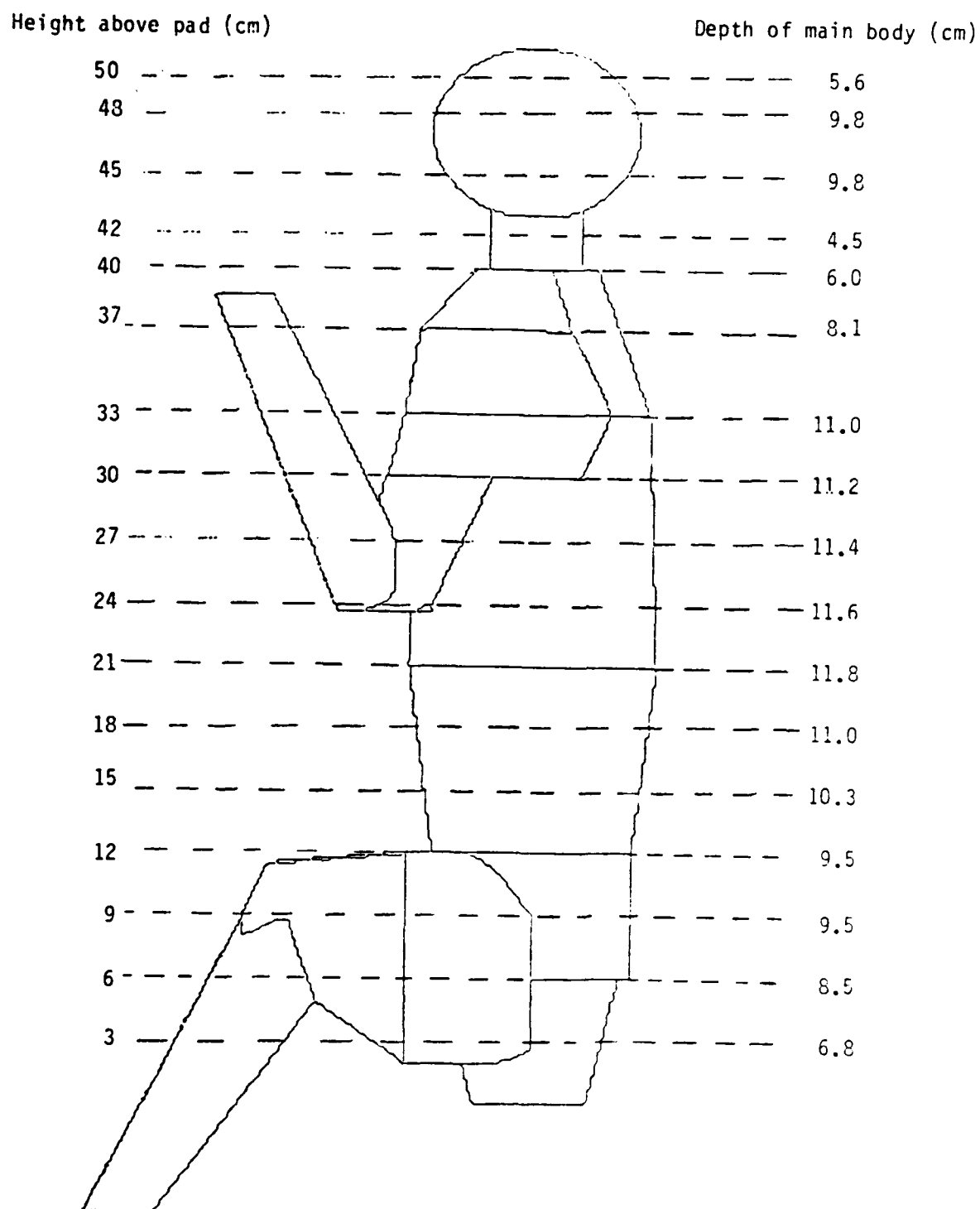
Figure 2. Location of cross sections, side view azimuth 90.0^{\circ} elevation 0.0^{\circ}
