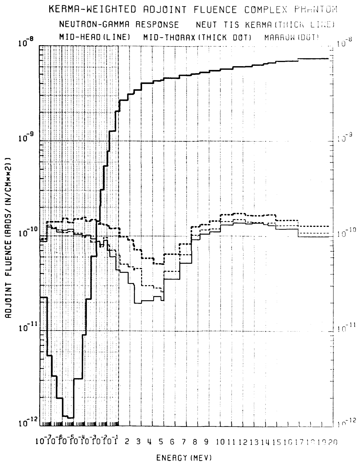
Figure 37. KERMA-weighted adjoint fluence complex phantom (n-g)
