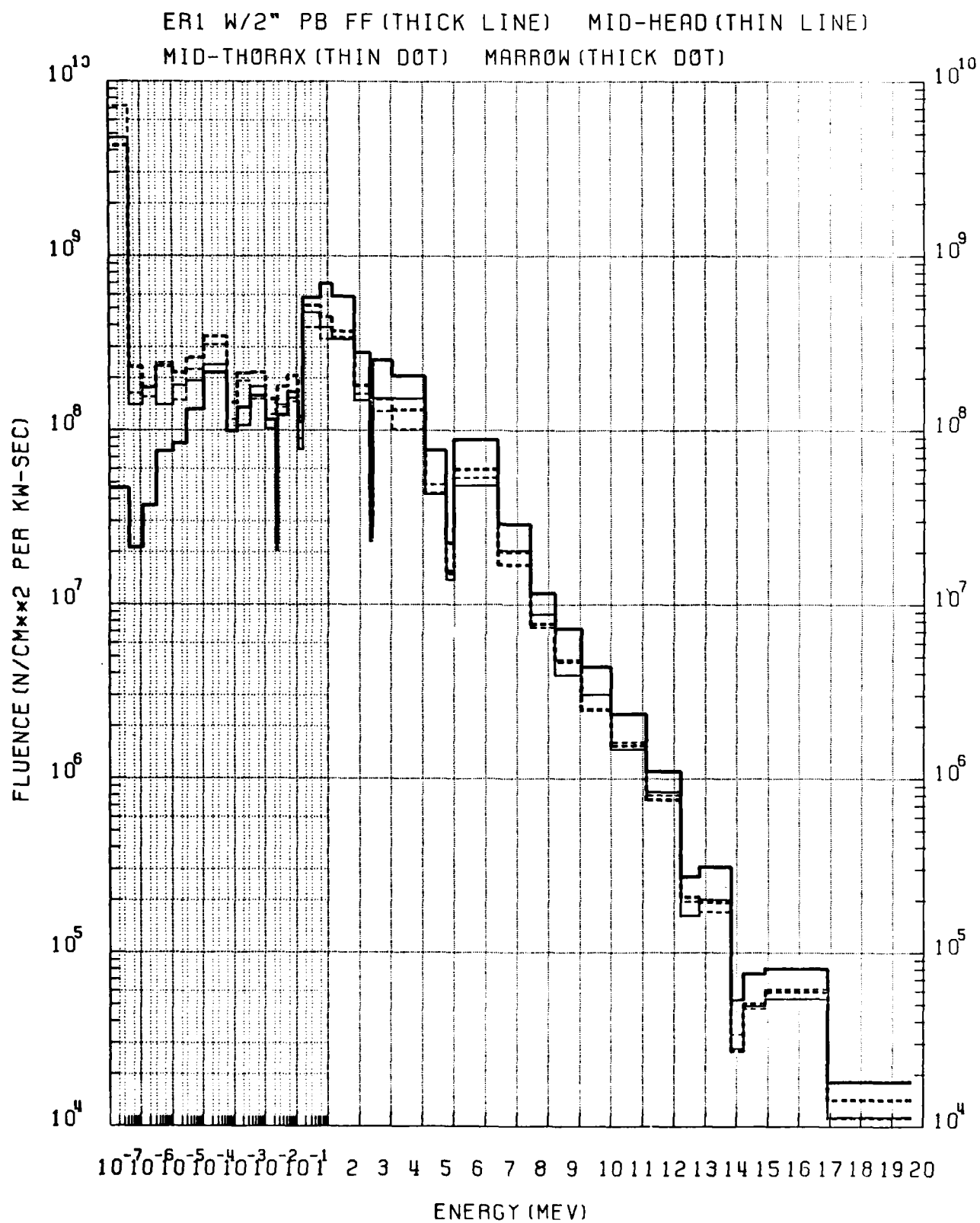
Figure 47. Neutron fluence for ER1 and complex phantom
