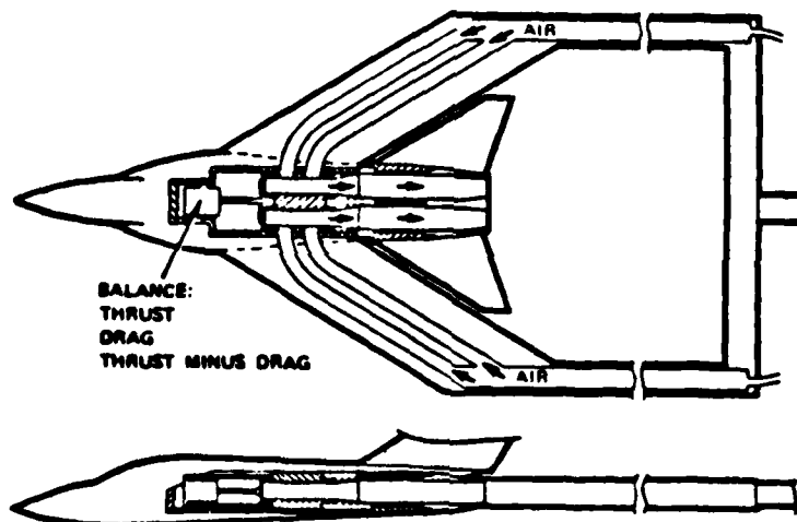
Figure 93. Tornado Afterbody Model (Reference 52)
