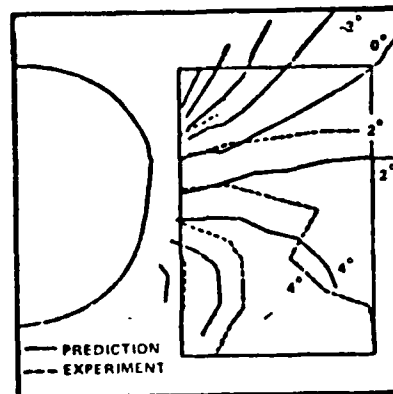
Figure 55. Inlet Flow Field Correlation for Side-Mounted Inlet: M = 2.5 , \alpha = 15 (Reference 32)
