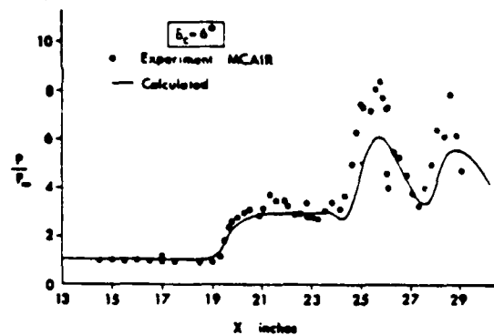
Static Pressure on Ramp for \delta_c = 6^\circ
