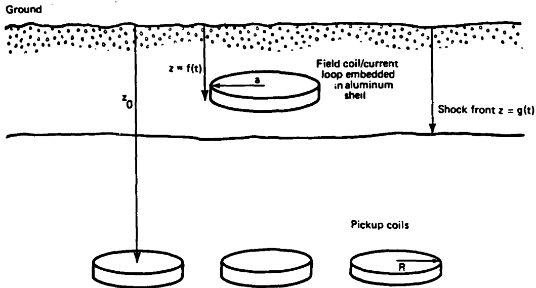
Figure 1. Gauge geometry.
