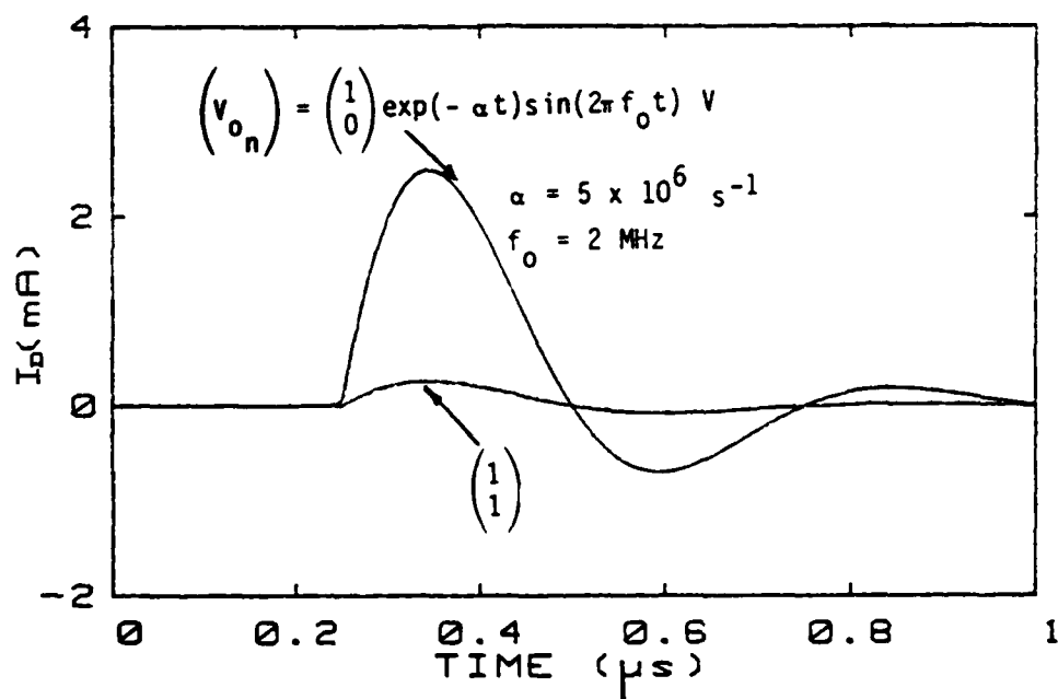
Figure B24. Common- and differential-mode currents ( I_B, I_D ) for different numbers of sources when \ell = 30 \text{ m} , x_s = 0.25 \text{ m} , x_m = 75 \text{ m} , Z_{\ell 11} = 100 \Omega , Z_{\ell 12} = 1 \Omega , and Z_{\ell 22} = 400 \Omega .
