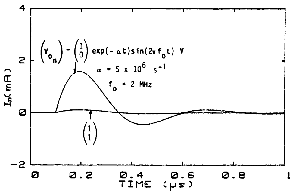
Figure B22. Common- and differential-mode currents ( I_B, I_D ) for different numbers of sources when \ell = 30 \text{ m} , x_s = 0.25 \text{ m} , x_m = 30 \text{ m} , Z_{\ell 11} = Z_{\ell 12} = Z_{\ell 22} = 400 \Omega .
