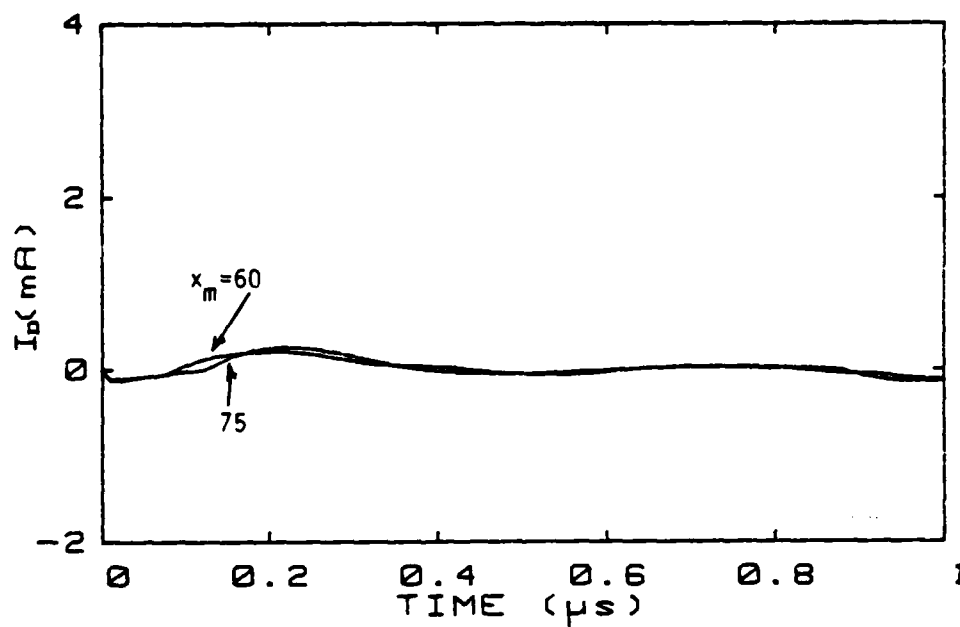
Figure B34. Common- and differential-mode currents ( I_B, I_D ) for different measurement locations when \ell = 75 m, x_s = 37.5 m, Z_{\ell 11} = 100 \Omega , Z_{\ell 12} = 1 \Omega , and Z_{\ell 22} = 400 \Omega .
