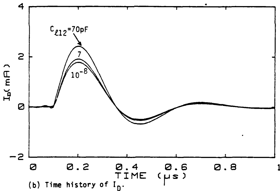
Figure 17. Common- and differential-mode currents ( I_B, I_D ) for different values of C_{L12} when \ell = 30 \text{ m} , x_s = 0.25 \text{ m} , x_m = 30 \text{ m} , Z_{L11} = 100 + 2\pi f j (3 \times 10^{-7}) + 1/[2\pi f j (7 \times 10^{-11})] \Omega , and Z_{L22} = 100 + 2\pi f j (2.5 \times 10^{-6}) \Omega .
