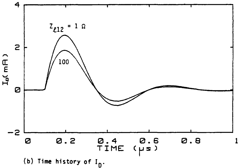
Figure B14. Common- and differential-mode currents ( I_B, I_D ) for different Z_{L12} when \ell = 30 \text{ m} , x_s = 0.25 \text{ m} , x_m = 30 \text{ m} , Z_{L11} = 10^4 \Omega , and Z_{L22} = 1 \Omega .
