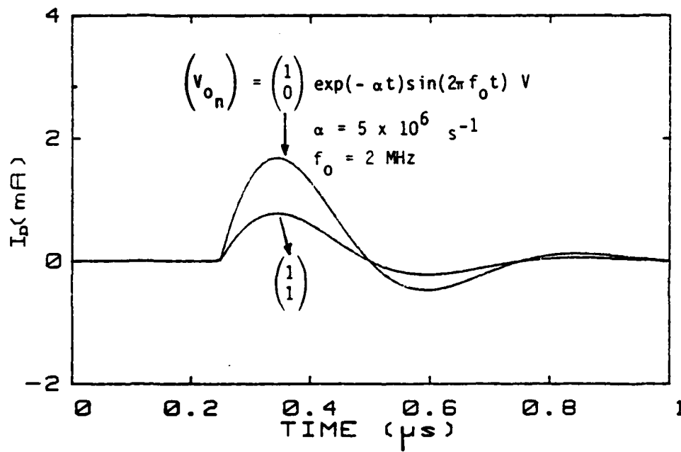
Figure B28. Common- and differential-mode currents ( I_B, I_D ) for different numbers of sources when \ell = 30 \text{ m} , x_s = 0.25 \text{ m} , x_m = 75 \text{ m} , Z_{\ell 11} = 100 \Omega , Z_{\ell 12} = \infty \Omega , and Z_{\ell 22} = 400 \Omega .
