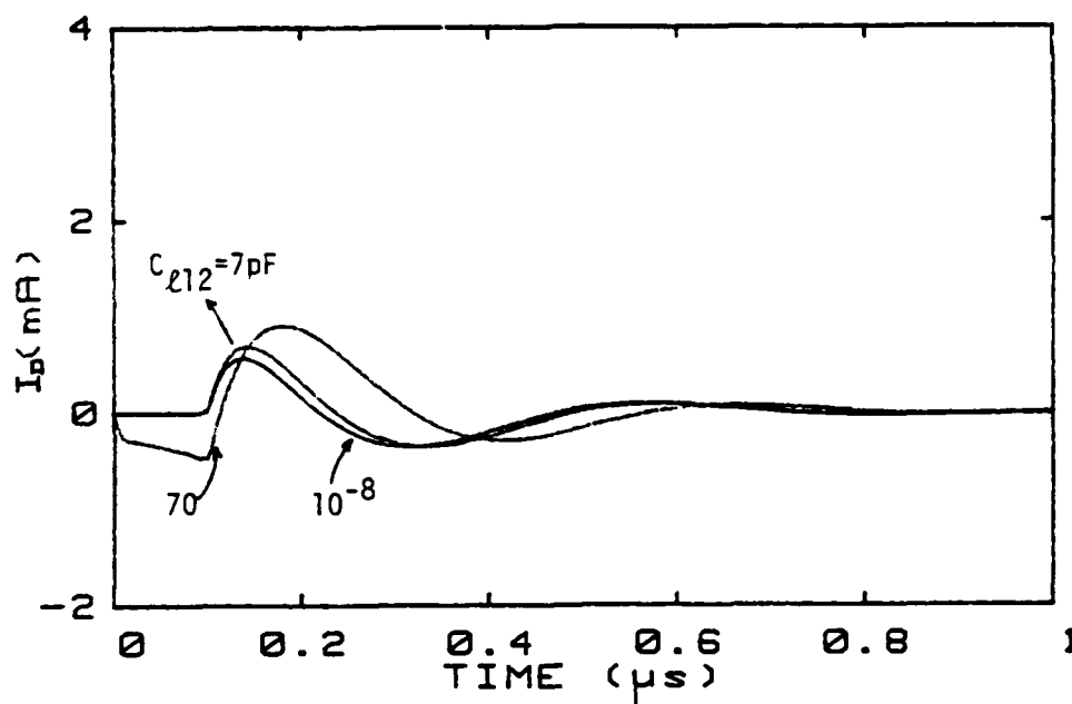
Figure B16. Common- and differential-mode currents ( I_B, I_D ) for different Z_{L12} when \ell = 30 \text{ m} , x_s = 0.25 \text{ m} , x_m = 30 \text{ m} , Z_{L11} = Z_{L22} = 100 + 2\pi f j (3 \times 10^{-7}) + 1/[2\pi f j (7 \times 10^{-11})] \Omega .
