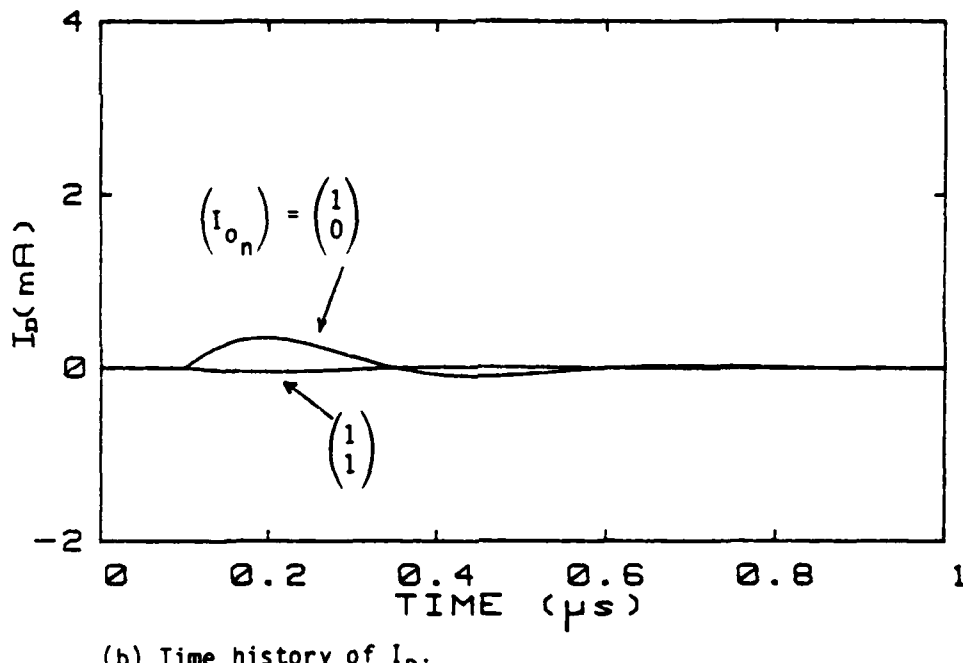
Figure 22. Common- and differential-mode currents ( I_B, I_D ) for different numbers of sources when \ell = 30 \text{ m} , x_s = 0.25 \text{ m} , x_m = 30 \text{ m} , Z_{\ell 11} = Z_{\ell 12} = Z_{\ell 22} = 400 \Omega .
