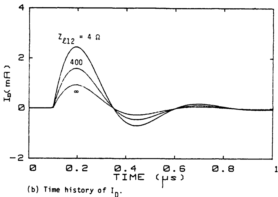
Figure 16. Common- and differential-mode currents ( I_B, I_D ) for different Z_{\ell 12} when \ell = 30 m, x_s = 0.25 m, x_m = 30 m and Z_{\ell 11} = Z_{\ell 22} = 400 \Omega .
