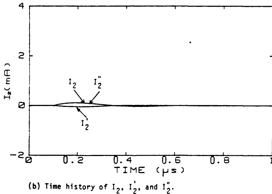
Figure 11. Exact wire currents ( I_1 , I_2 ) and estimated wire currents ( I_1' , I_2' ; I_1'' , I_2'' ) using two variational principle techniques when \ell = 30 \text{ m} , x_s = 0.25 \text{ m} , x_m = 30 \text{ m} , Z_{\ell 11} = Z_{\ell 12} = Z_{\ell 22} = 400 \Omega .
