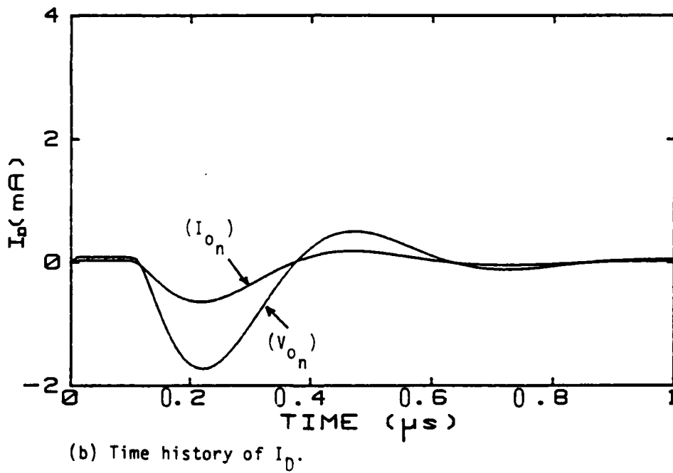
Figure 18. Common- and differential-mode currents ( I_B, I_D ) for different types of sources when \ell = 30 \text{ m} , x_s = 0.25 \text{ m} , x_m = 30 \text{ m} , Z_{\ell 11} = Z_{\ell 22} = 2\pi f j(3 \times 10^{-7}) + 1/[2\pi f j(7 \times 10^{-11})] \Omega , and Z_{\ell 12} = 1/[2\pi f j(7 \times 10^{-12})] \Omega .
