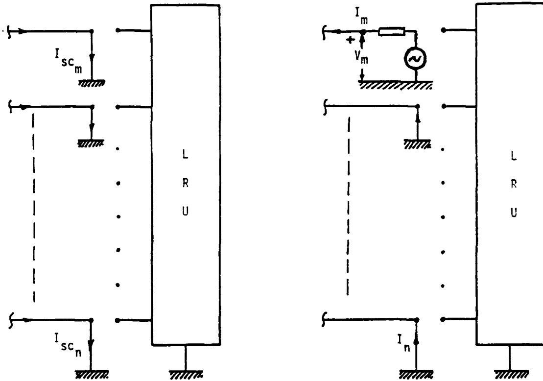
(a) Short-circuit currents
