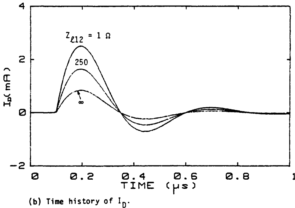
Figure B13. Common- and differential-mode currents ( I_B, I_D ) for different Z_{L12} when \ell = 30 m, x_s = 0.25 m, x_m = 30 m, Z_{L11} = 500 \Omega , and Z_{L22} = 100 \Omega .
