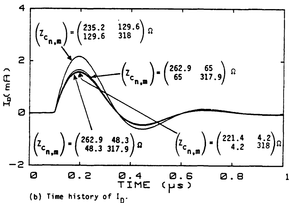
Figure 23. Common- and differential-mode currents ( I_B, I_D ) for different characteristic impedances when \ell = 30 m, x_s = 0.25 m, x_m = 30 m, Z_{\ell 11} = Z_{\ell 12} = Z_{\ell 22} = 400 \Omega , and (Z_{o_{n,m}}) = (Z_{c_{n,m}}) .
