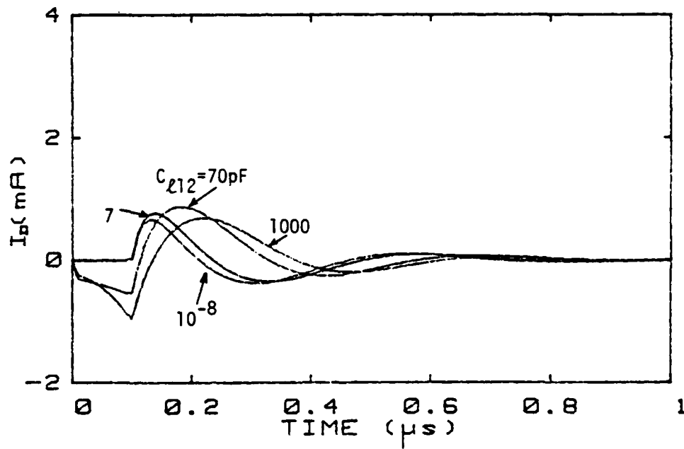
Figure B17. Common- and differential-mode currents ( I_B, I_D ) for different Z_{L12} when \ell = 30 \text{ m} , x_s = 0.25 \text{ m} , x_m = 30 \text{ m} , and Z_{L11} = Z_{L22} = 2\pi f j (3 \times 10^{-7}) + 1/[2\pi f j (7 \times 10^{-11})] \Omega .
