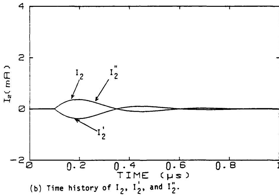
Figure 10. Exact wire currents ( I_1 , I_2 ) and estimated wire currents ( I_1' , I_2' , I_1'' , I_2'' ) using two variational principle techniques when \ell = 30 \text{ m} , x_s = 0.25 \text{ m} , x_m = 30 \text{ m} , Z_{\ell 11} = Z_{\ell 12} = Z_{\ell 22} = 400 \Omega .
