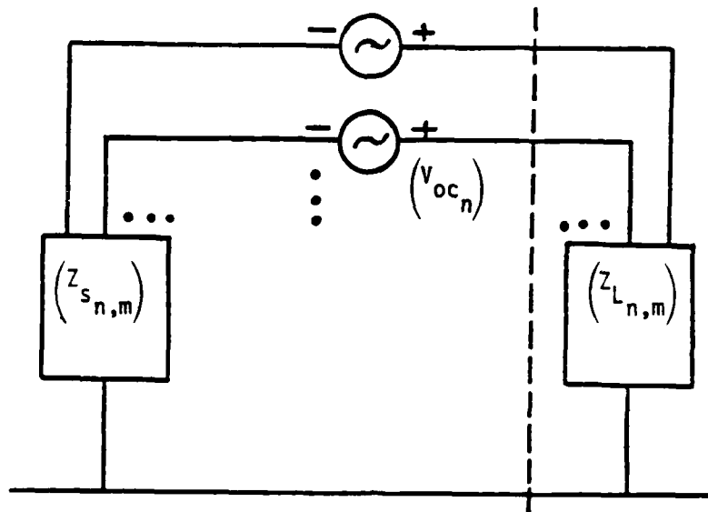
(a) The Thévenin equivalent circuit.
