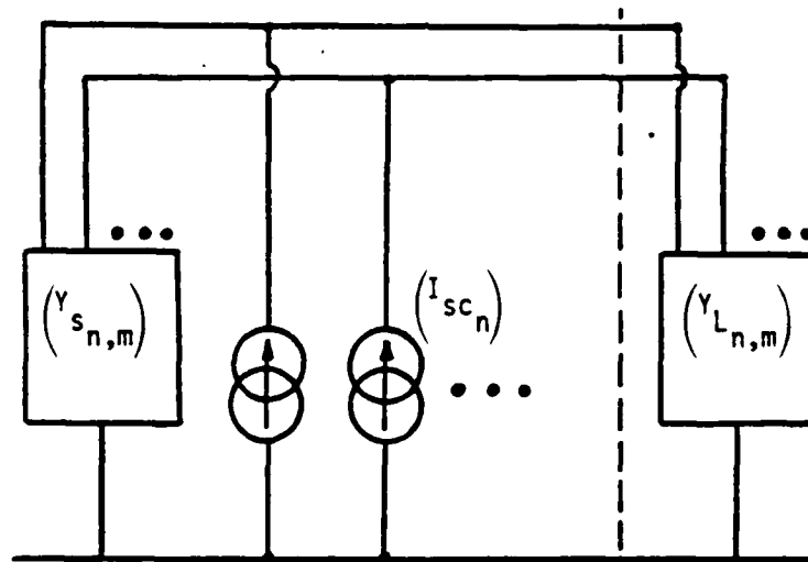
(b) The Norton equivalent circuit
