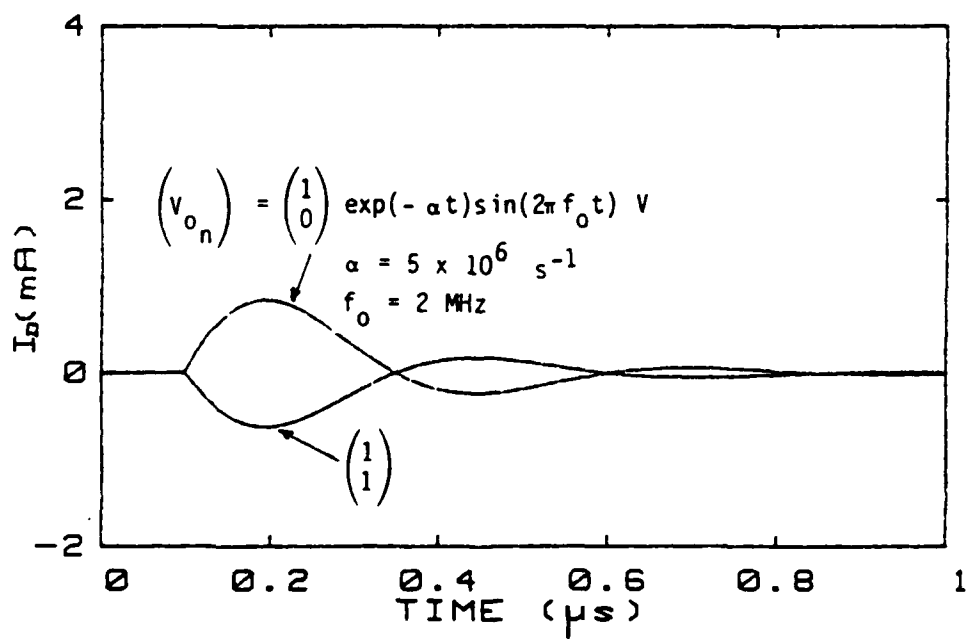
Figure B29. Common- and differential-mode currents ( I_B, I_D ) for different numbers of sources when \ell = 30 \text{ m} , x_s = 0.25 \text{ m} , x_m = 30 \text{ m} , Z_{\ell 11} = 500 \Omega , Z_{\ell 12} = \infty , and Z_{\ell 22} = 100 \Omega .
