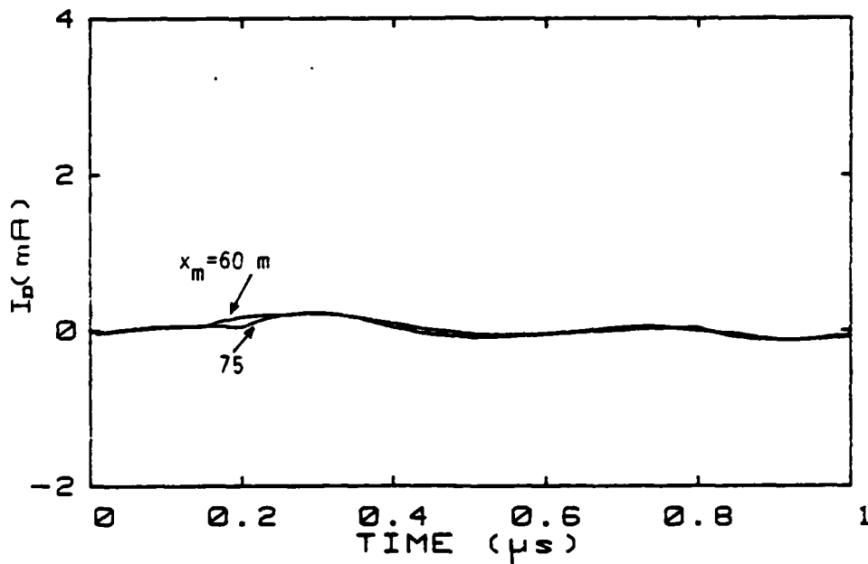
Figure B33. Common- and differential-mode currents ( I_B, I_D ) for different measurement locations when \ell = 75 \text{ m} , x_s = 15 \text{ m} , Z_{\ell 11} = 100 \Omega , Z_{\ell 12} = 1 \Omega , Z_{\ell 22} = 400 \Omega .
