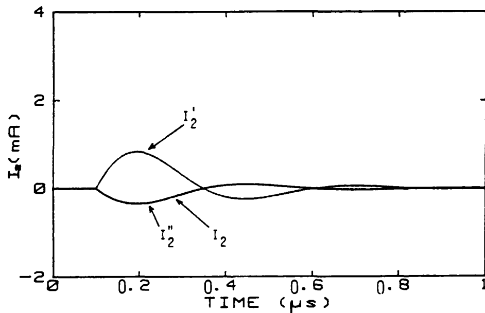
Figure B8. Exact wire currents ( I_1 , I_2 ) and estimated wire currents ( I_1' , I_2' ; I_1'' , I_2'' ) using two variational principle techniques when \ell = 30 \text{ m} , x_s = 0.25 \text{ m} , x_m = 30 \text{ m} , Z_{\ell 11} = 1 \Omega , Z_{\ell 12} = 1 \Omega and Z_{\ell 22} = 10^4 \Omega .
