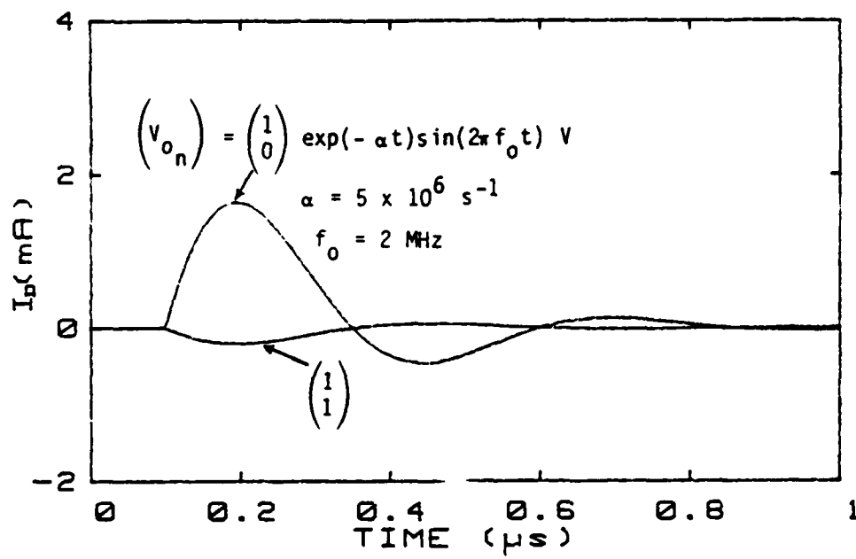
Figure B23. Common- and differential-mode currents ( I_B, I_D ) for different numbers of sources when \ell = 30 \text{ m} , x_s = 0.25 \text{ m} , x_m = 30 \text{ m} , Z_{\ell 11} = 500 \Omega , Z_{\ell 12} = 250 \Omega , Z_{\ell 22} = 100 \Omega .
