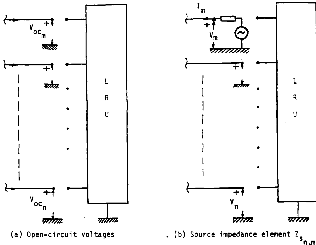
Figure 3. Experimental setups to measure the open-circuit voltages and the source impedance element Z_{s_{n,m}} .
