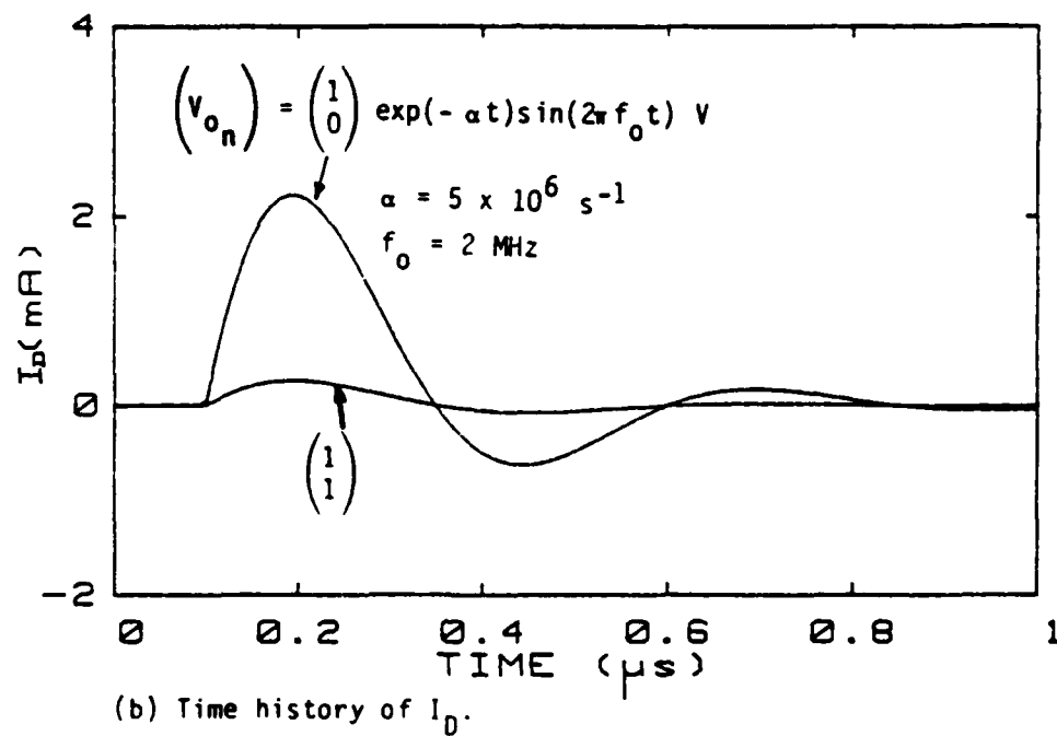
Figure 20. Common- and differential-mode currents ( I_B, I_D ) for different numbers of sources when \ell = 30 m, x_s = 0.25 m, x_m = 30 m, Z_{\ell 11} = Z_{\ell 12} = Z_{\ell 22} = 100 \Omega .
