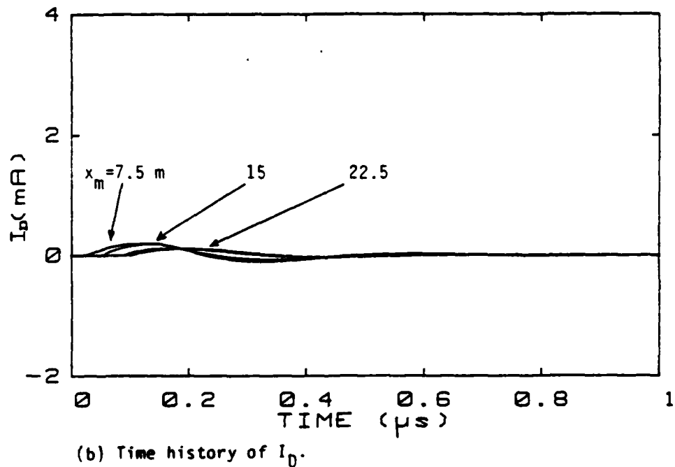
Figure B32. Common- and differential-mode currents ( I_B, I_D ) for different measurement locations when \ell = 30 m, x_s = 0.25 m, Z_{\ell 11} = Z_{\ell 12} = Z_{\ell 22} = 400 \Omega .
