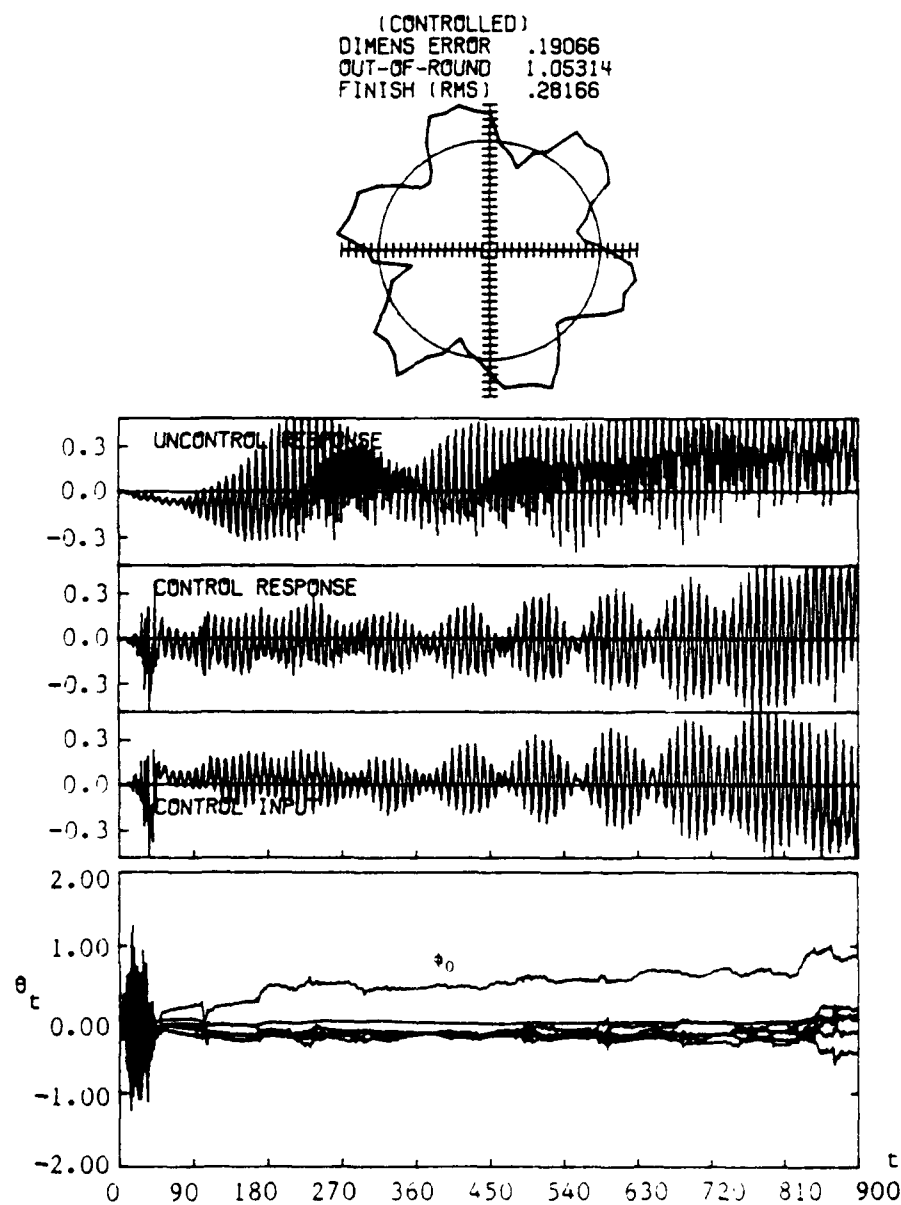
Figure 6.7 FCC for Machining process With Less Rigid Structure
