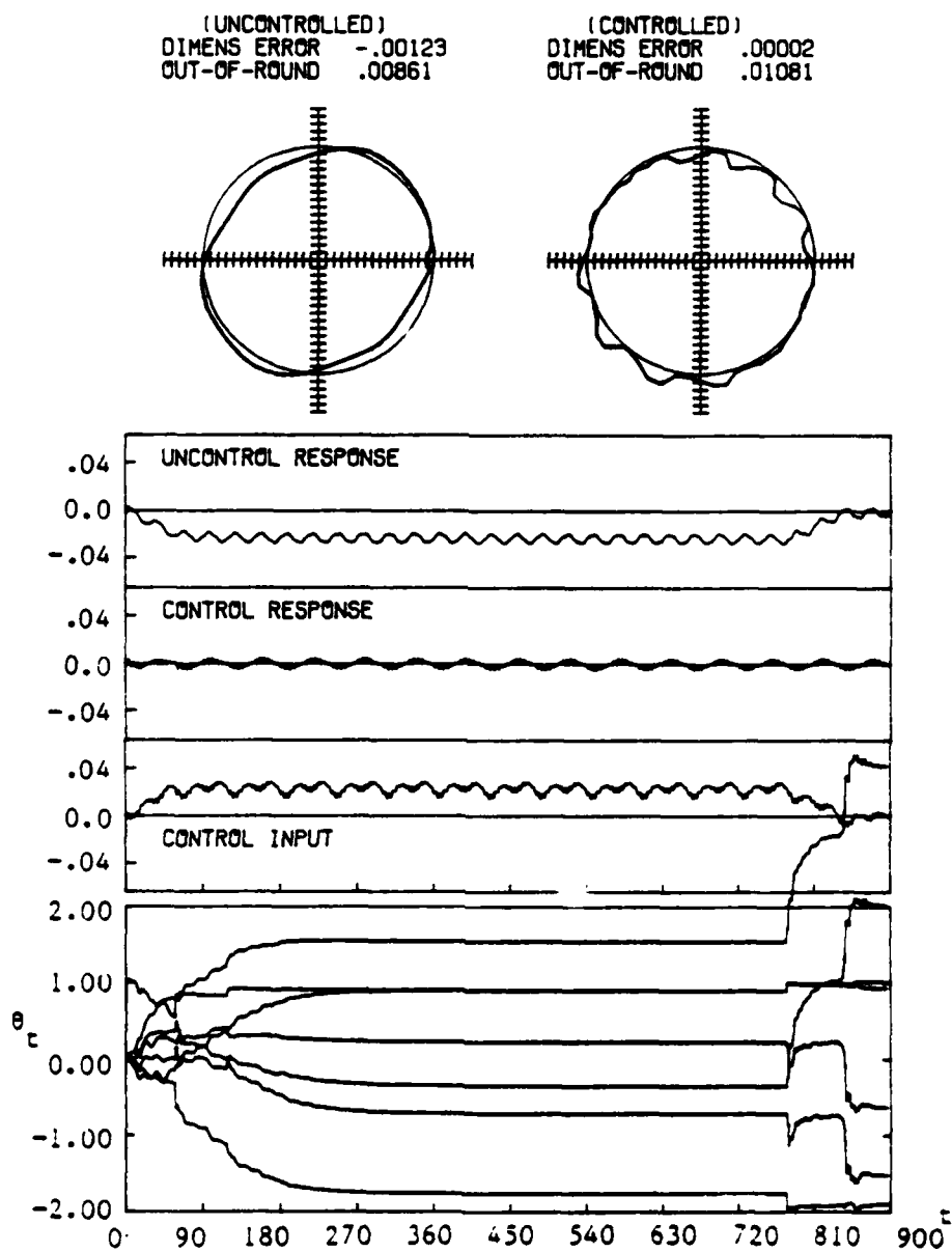
Figure 5.13 GAC System With Multiprobe Measurement and Periodic Disturbance (Simulation II-1)
