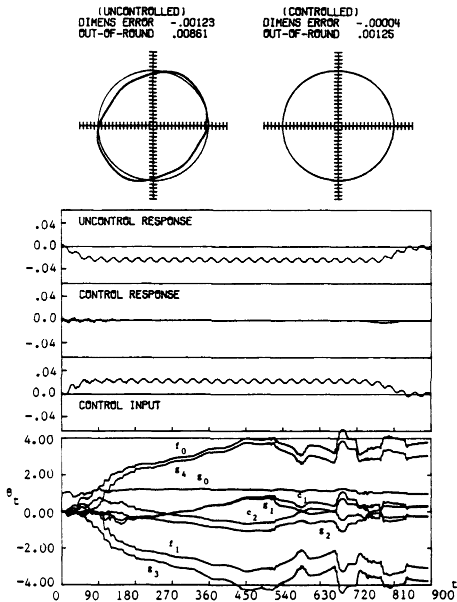
Figure 5.8 Perturbation Input for GAC System With Large Time Delay (Simulation I-6)
