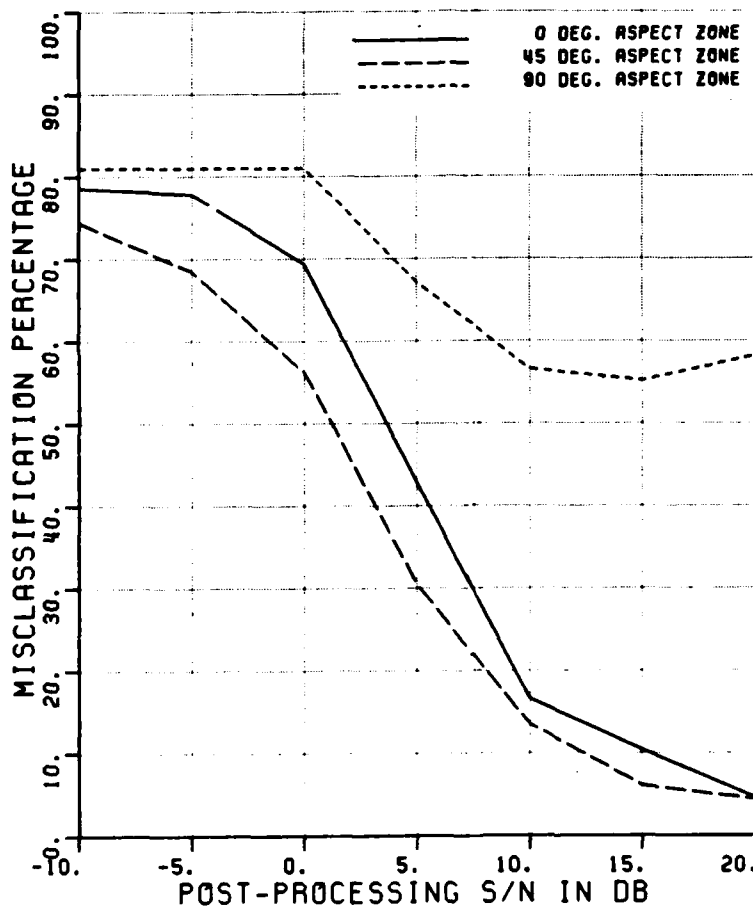
Figure A.71 Misclassification percentage versus post-processing SNR, comparing the performance of various aspect zones, with a forced error in aspect angle.
