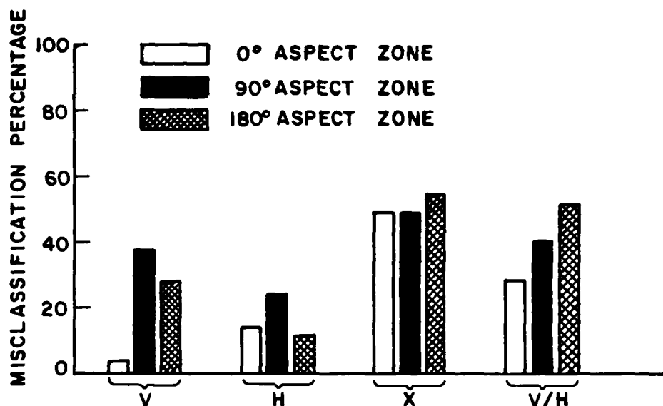
Figure 6.35. Average difference in misclassification percentage at 10 dB post-processing SNR between classifications having a 0° aspect error and classifications having a ±10° aspect error, at various aspect zones, as a function of polarization.
