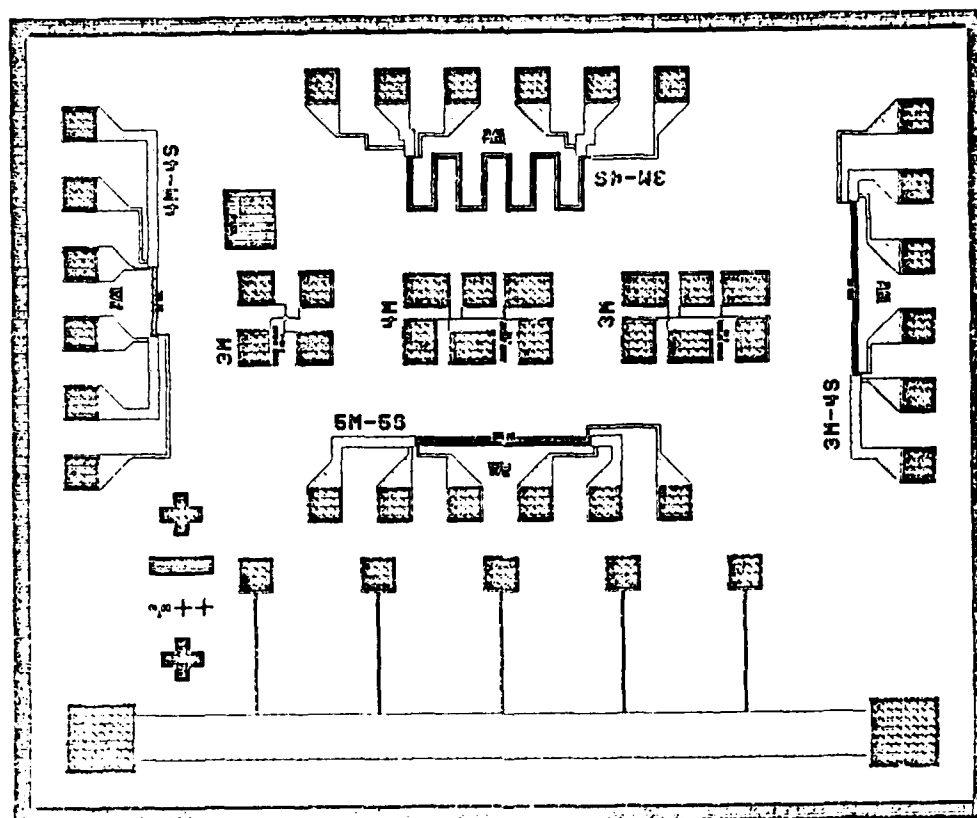
Figure 15. Electromigration Test Pattern
