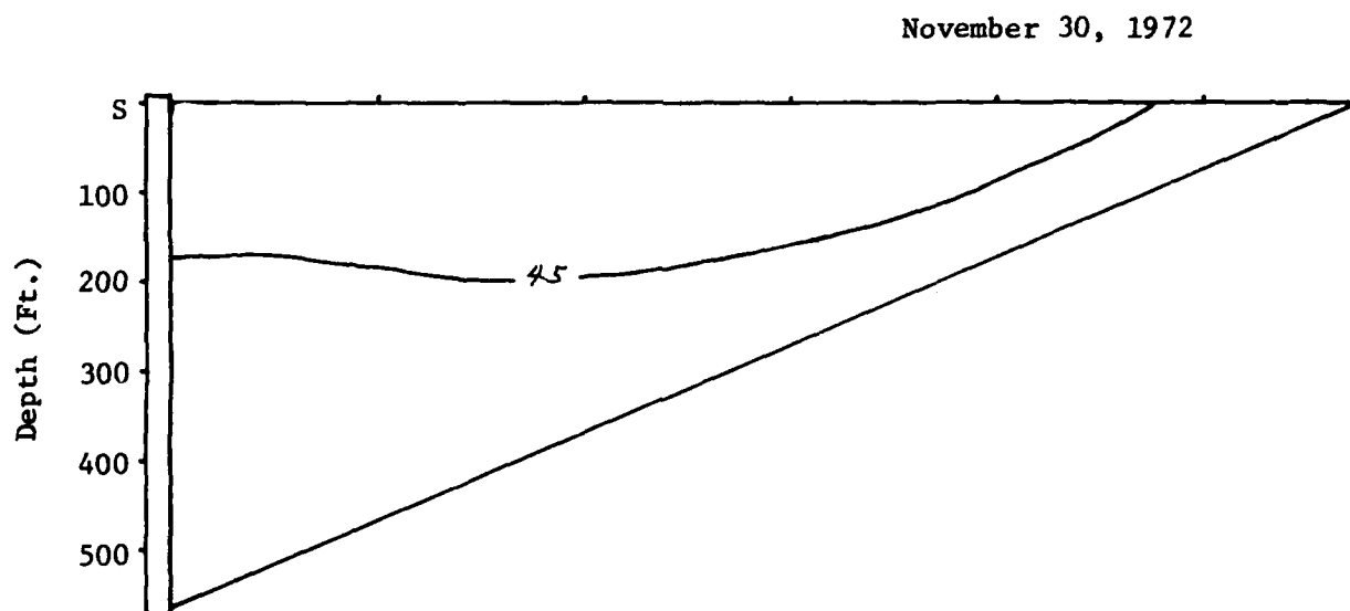
Figure 7. Longitudinal temperature profiles (F) in Dworshak Reservoir, 1972.
