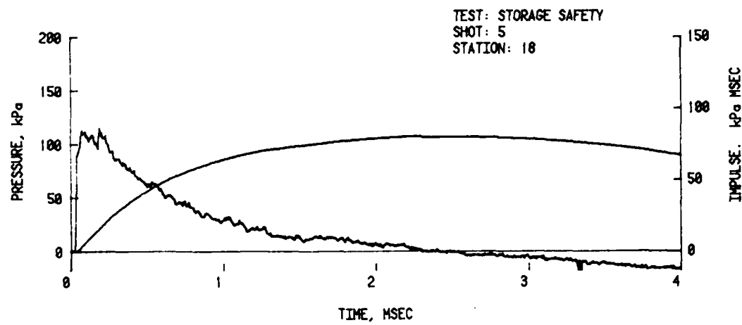
Figure 18. Pressure-Time Records from Front End Wall, Station 18
