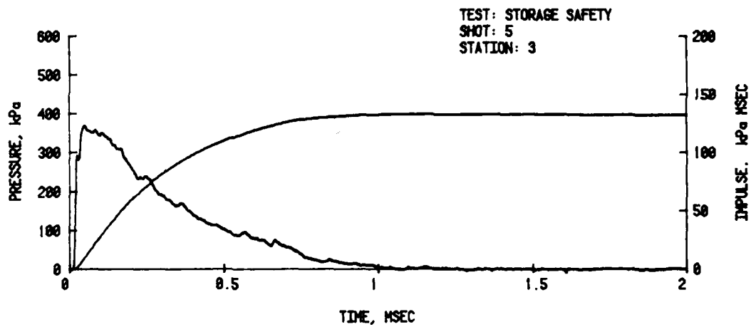
Figure 13. Pressure-Time Records from Near Side-Wall, Station 3
