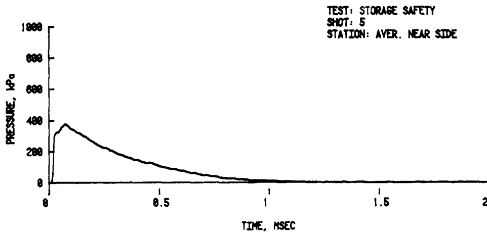
Figure 23. Average Loading on Near Side-Wall
