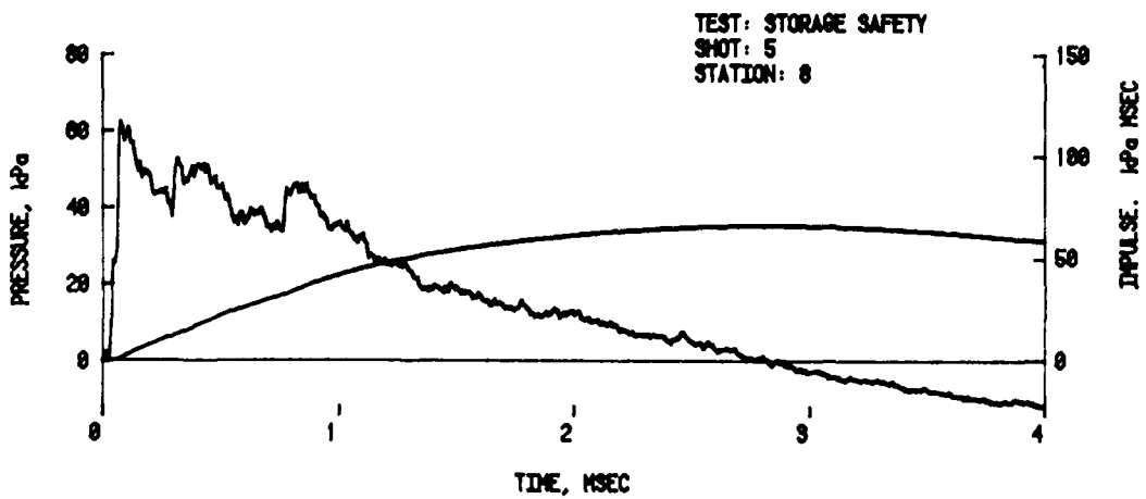
Figure 19. Pressure-Time Records from Far Side-Wall, Station 8
