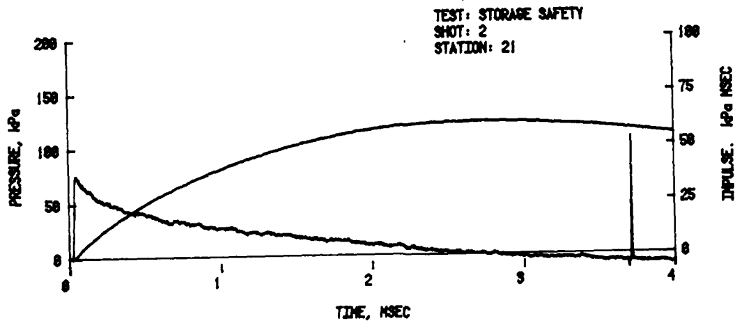
Figure 11. Pressure-Time Records, Free-Field with Barricades (Cont.)
