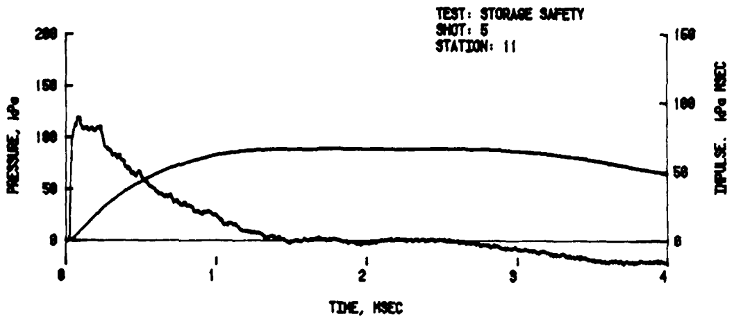
Figure 17. Pressure-Time Records from Back End-Wall, Station 11
