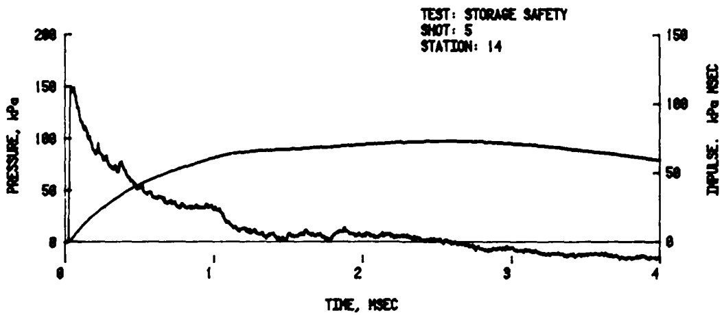
Figure 15. Pressure-Time Records from the Roof, Station 14
