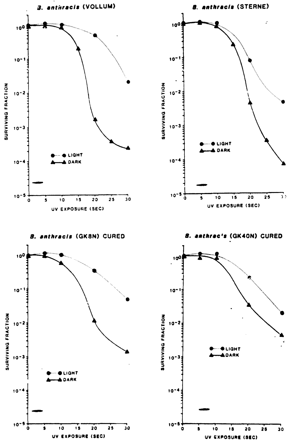
FIG. 4. UV-inactivation and photoreactivation of four strains of B. anthracis . Survival with photoreactivation light (●) and in the dark (▲) as a function of UV dose.
