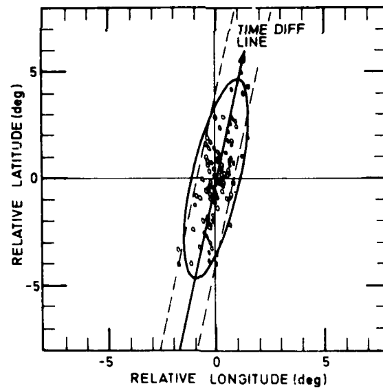
Fig. VII.8.3 Simulated 2-array (or two 3-comp. stations) event locations at 45.3^\circ\text{N} ; 149.3^\circ\text{E} for NORSAR and LASA. In case a) only azimuth observations are used ( \sigma = 2^\circ ), while in case b) further constraints are added by using P arrival time differences ( \sigma = 2.0 sec).
