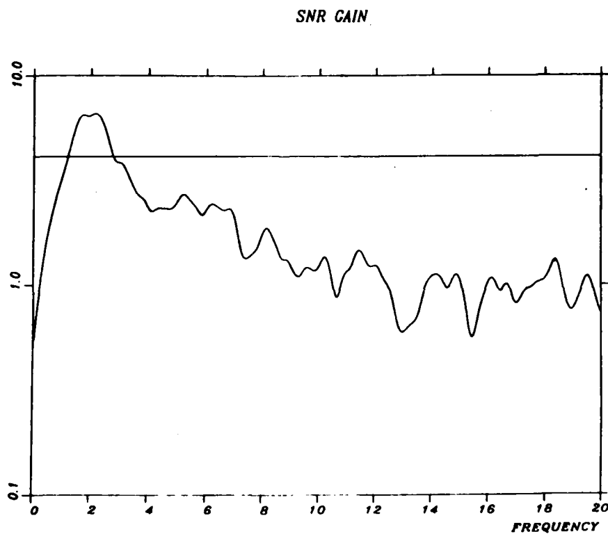
Fig. VII.2.7 Beamforming gain for array "TELEV" for P-arrival from Novaja Zemlja event. P-wave data analysis window on top. The horizontal line in the gain plot indicates \sqrt{N} gain, with N = 17 for this subgeometry.
