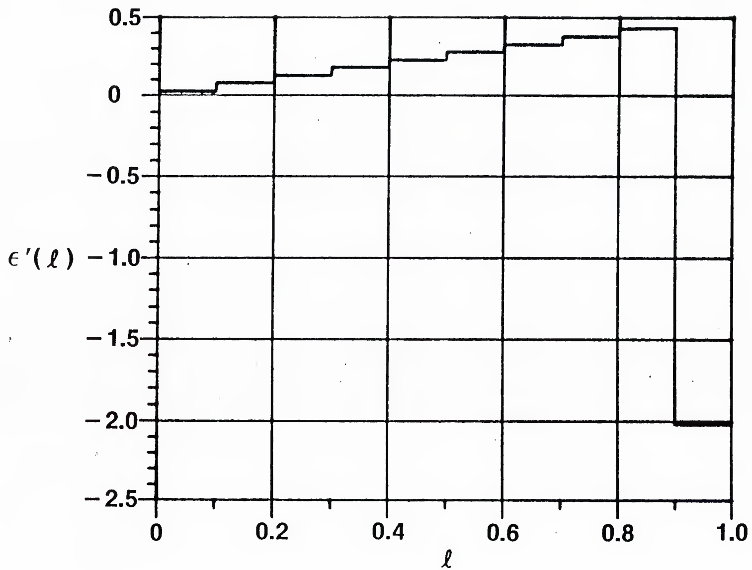
Figure 20. Shear Diagram
