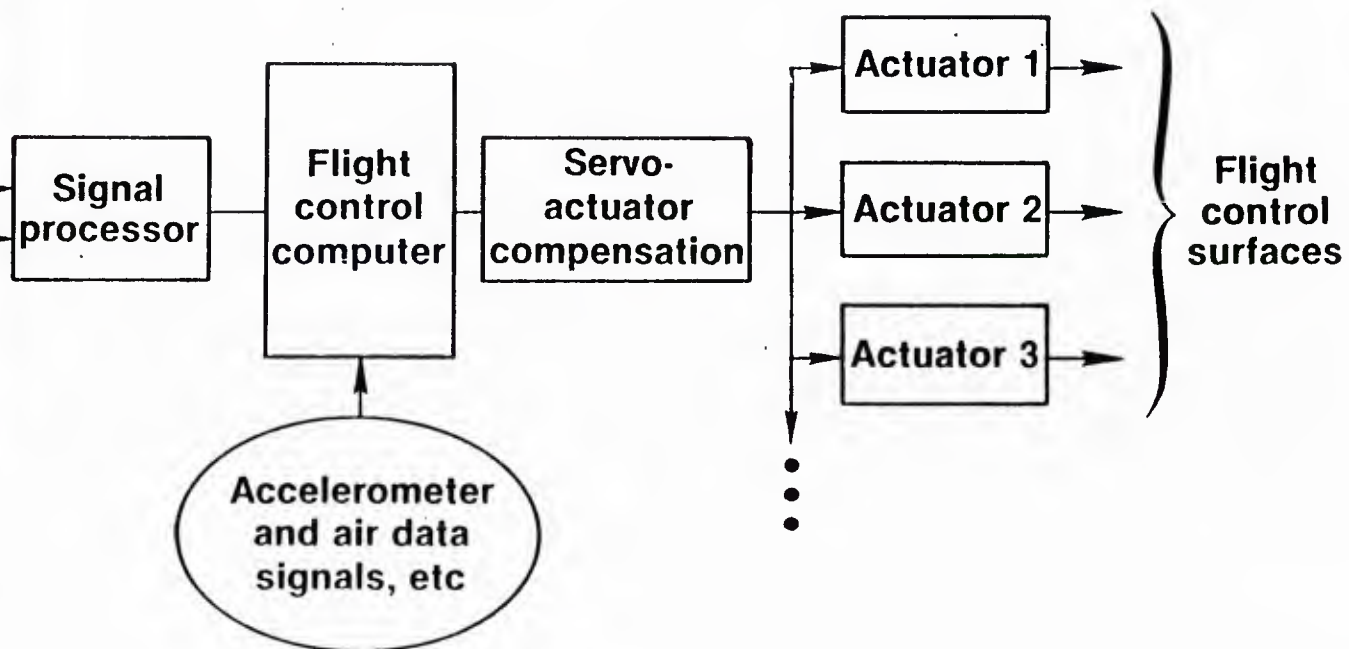
Figure 2. Wing Load Compensation
