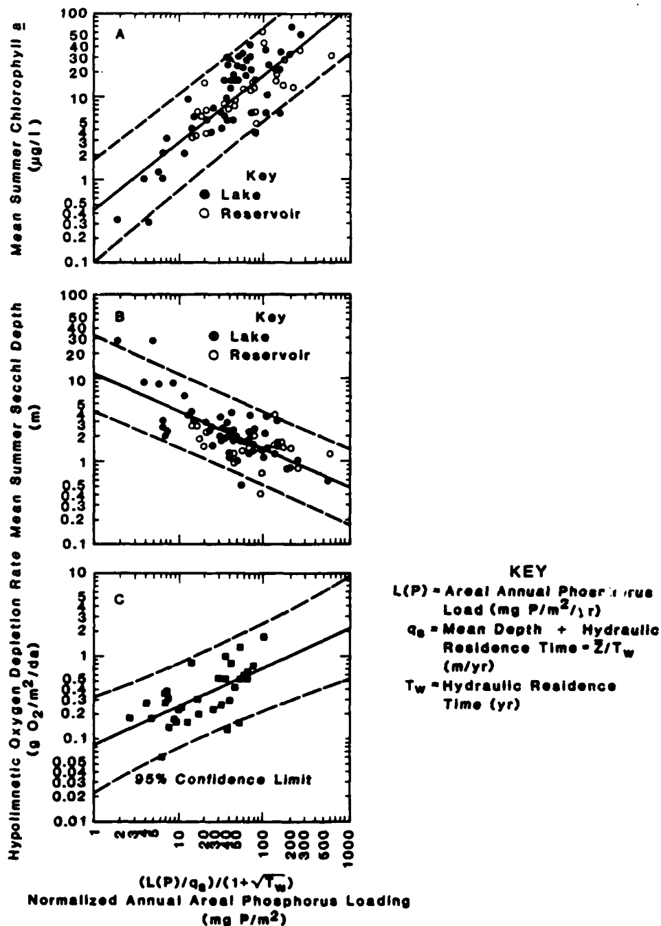
Figure 4. Updated P load-eutrophication-related water quality response relationships for U.S. Water bodies. (Reprinted with permission from J. Water Research , Vol 16, R. A. Jones and G. F. Lee, "Recent Advances in Assessing the Impact of Phosphorus Loads in Eutrophication-Related Water Quality," 1982, Pergamon Press, Ltd.)
