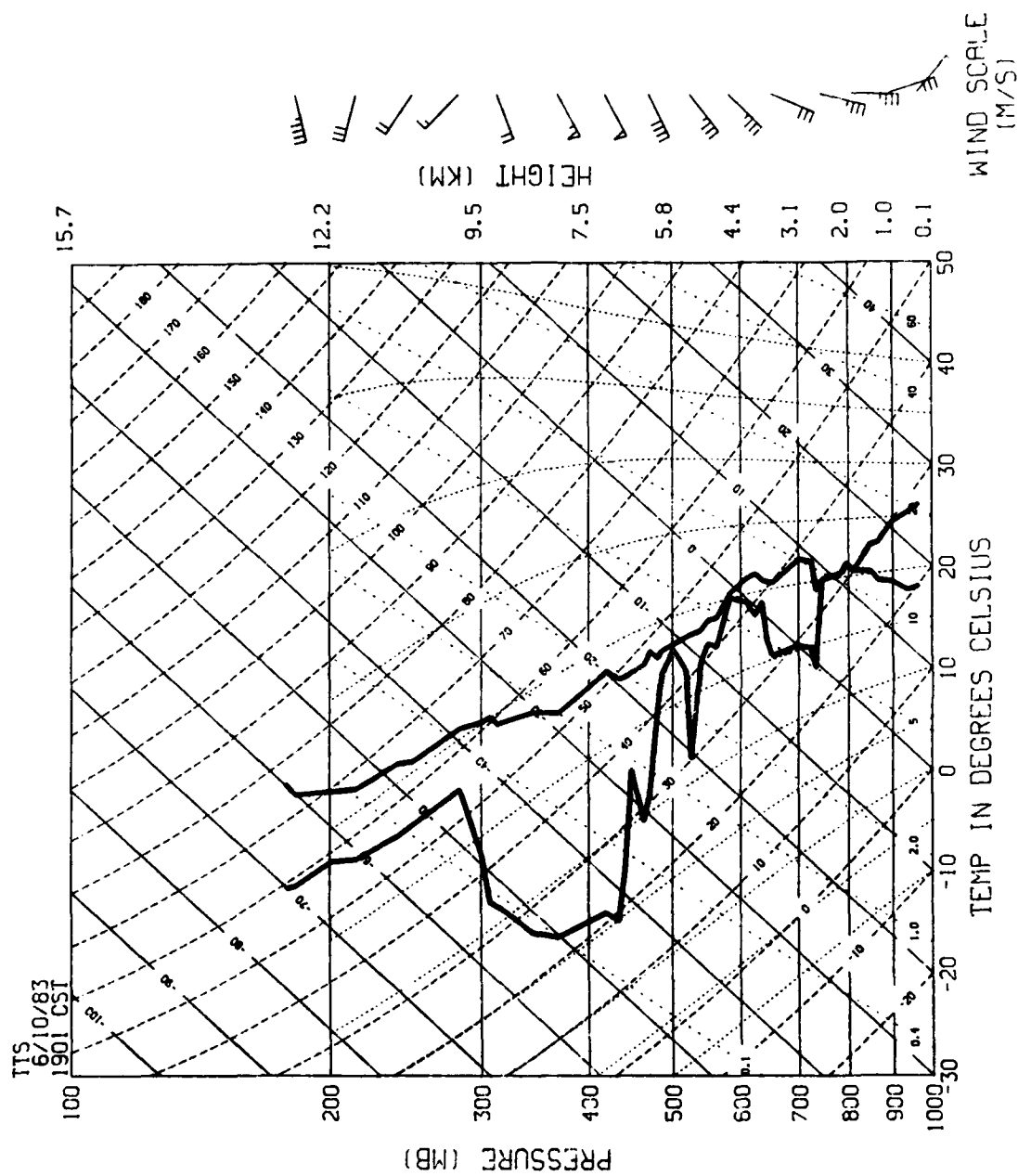
Fig. IV-7(e). Thermodynamic sounding taken at Tuttle (TTS), OK at 1901 CST on 10 June 1983.
