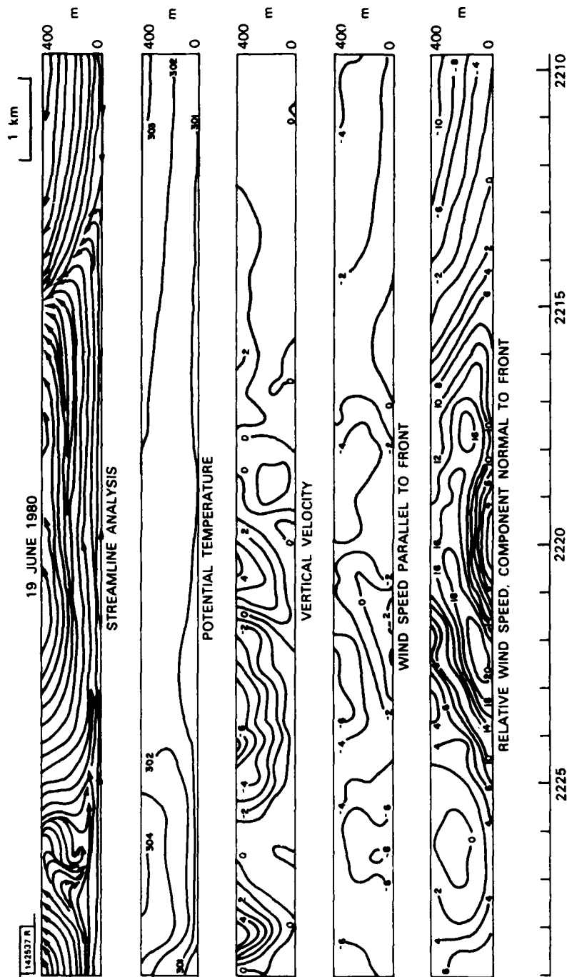
Fig. IV-3(e). Plots of WKY-TV tower data collected during the passage of the gust front (2210-2229 CST) on 19 June 1980.
