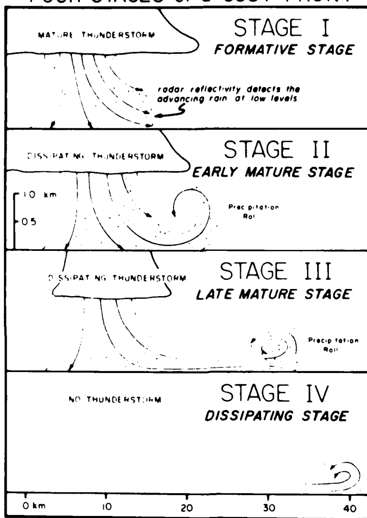
Fig. II-3. Life cycle of the gust front (vertical cross section). Note the formation of the "precipitation roll" which is believed to produce the thin line echo.
