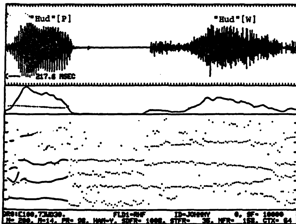
Figure 5. A digital spectrogram [SGM] with formant tracking [FTR] for an adult male speaker's production of a phonated [P] and whispered [W] vowel /ʌ/ embedded in the word "Hud".
