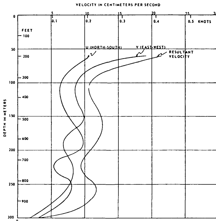
MEAN CURRENT VELOCITIES VERSUS DEPTH FOR DECEMBER-JANUARY TEST PERIOD OFF SANTA CATALINA
