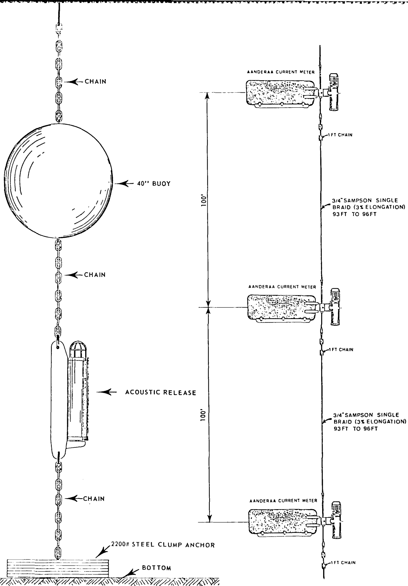
BOTTOM ELEMENTS OF THE CURRENT METER STRING AND METER CONNECTION DETAILS
