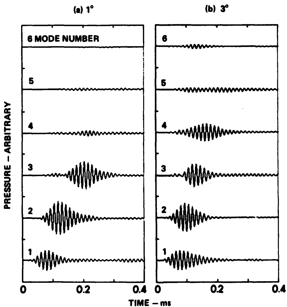
FIGURE 5 NORMAL MODE WAVEFORMS AT BOTTOM SLOPES OF (a) 1^\circ AND (b) 3^\circ AT RANGE OF 4 m THE SOURCE IS NEAR THE SURFACE IN 5 cm OF WATER AND PROPAGATION IS DOWNSLOPE
