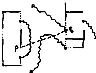
Figure 3. A portion of a sketch with a cut \overline{pq} . The flow across \overline{pq} is 1.
