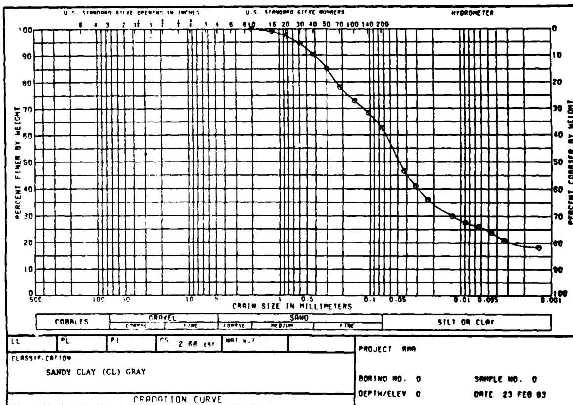
Figure 3. Grain-size distribution of RMA soil used as an adsorbent
