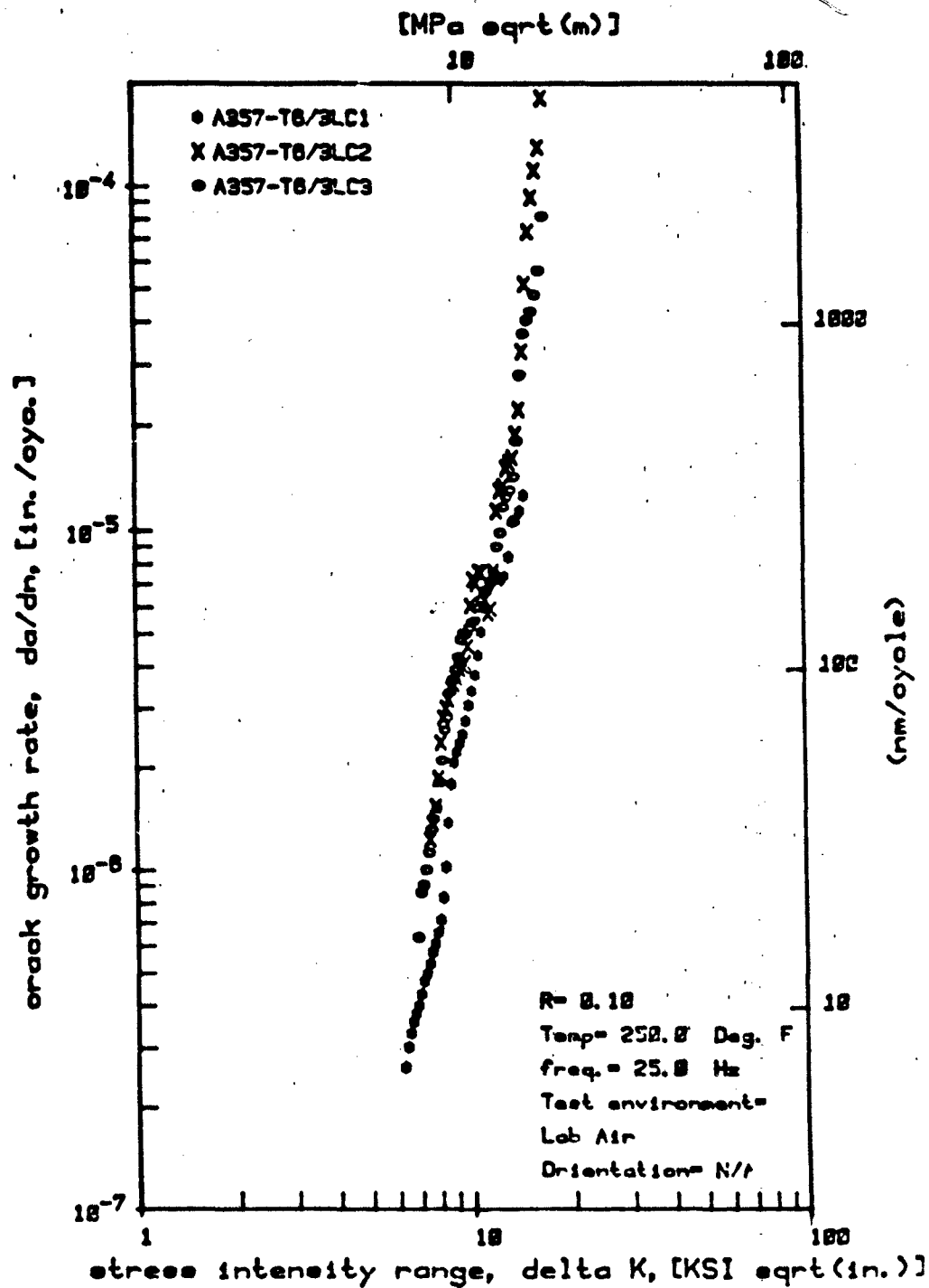
Figure 10: A357-T6 Fatigue Crack Growth Rate Data at 250 o F.
