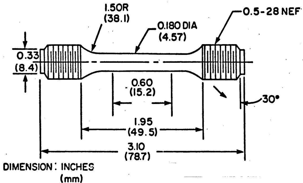
Figure 3: Fatigue test specimen.
