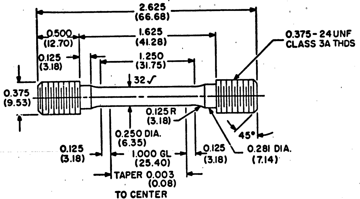
Figure 2: Tensile test specimen.
