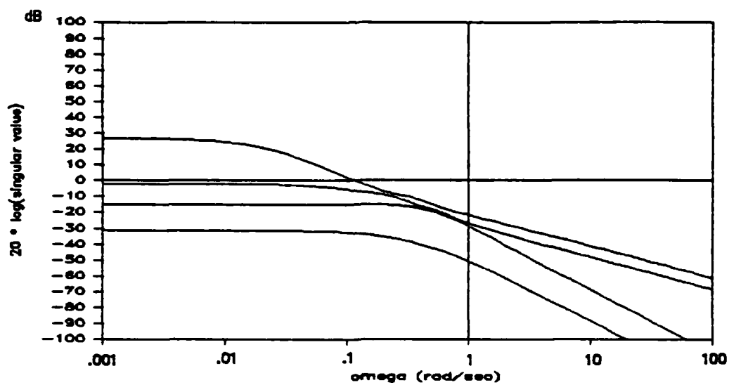
(a) Unaugmented Plant
