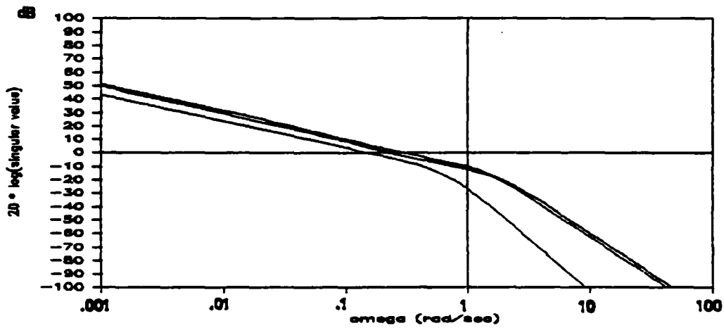
(e) Recovered Open Loop Transfer Function, G(s)K(s)
