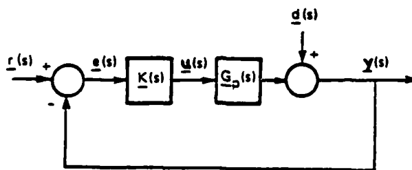
Figure 4.1 Block Diagram of a MIMO Compensated Plant
