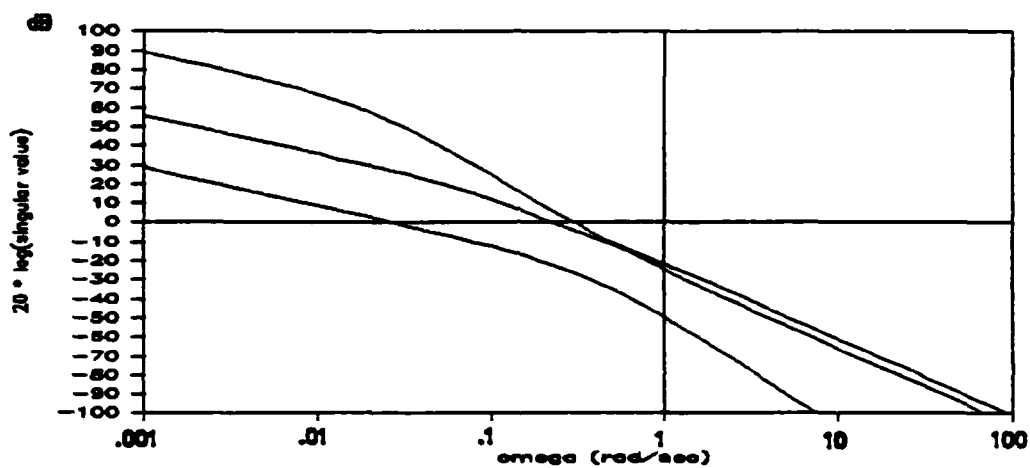
(b) Augmented Open Loop Plant
