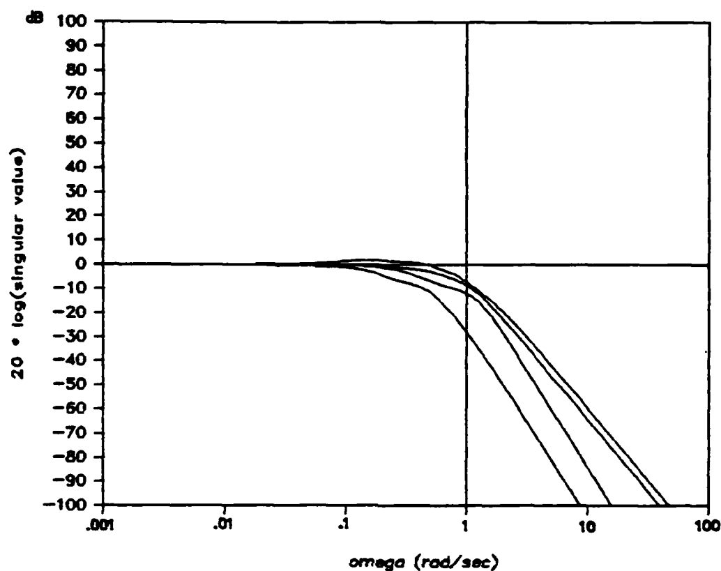
Figure 4.8 Singular Values of the Closed Loop
