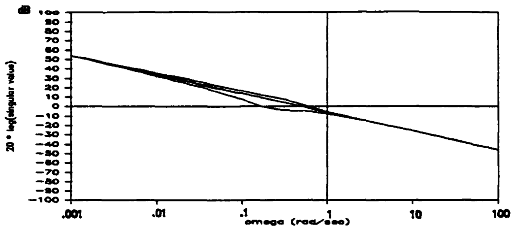
(a) Kalman Filter Open Loop, G_{FOL}
