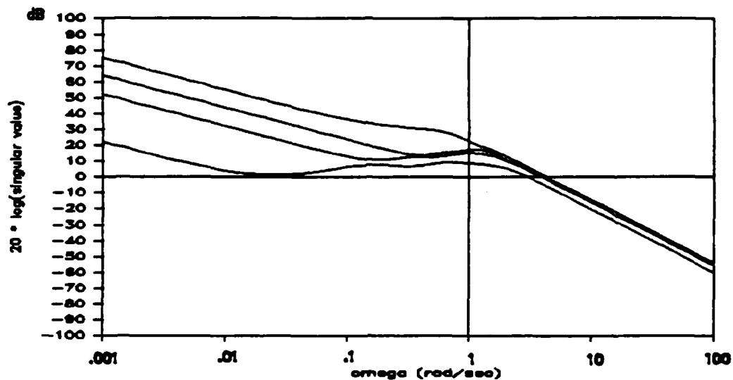
Figure 4.9 Compensator Singular Values
