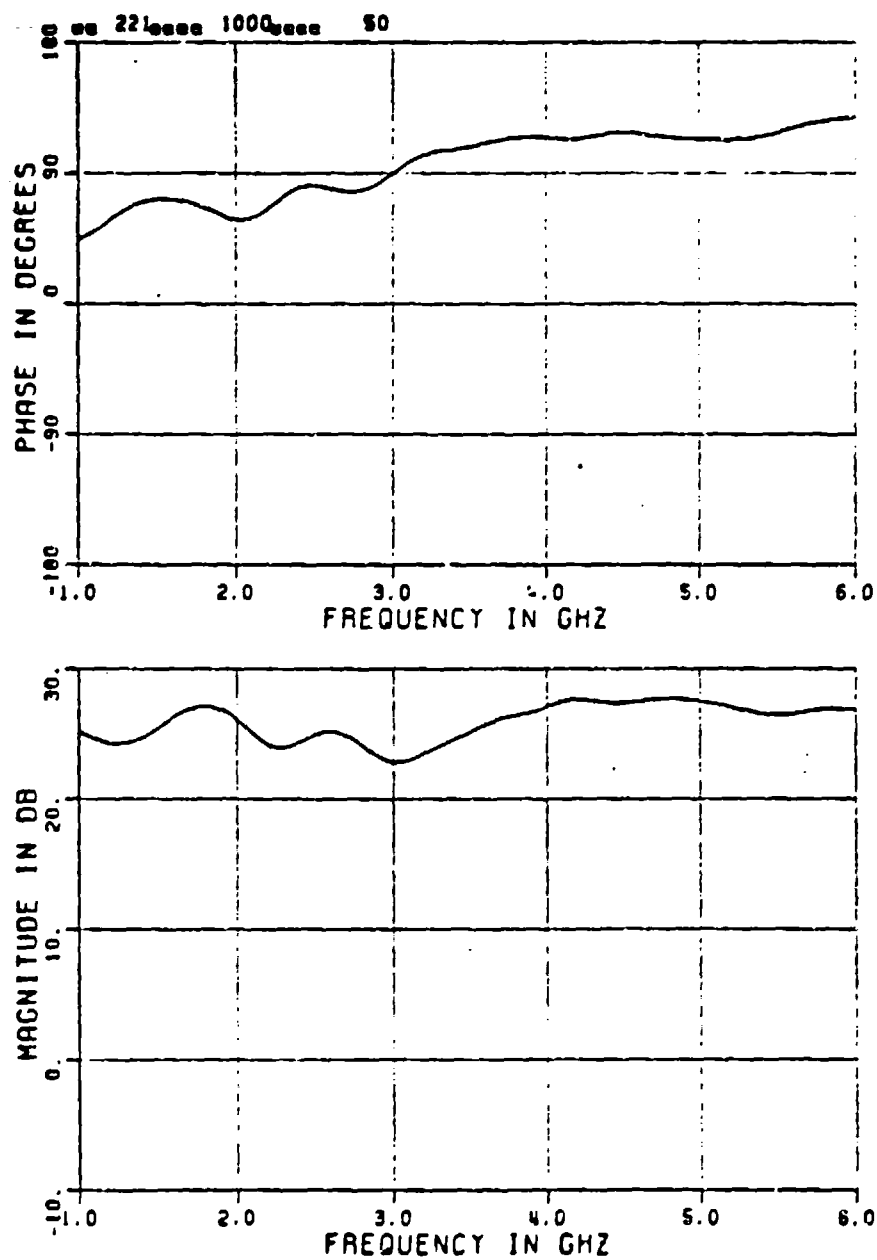
Figure 4.6. Horizontally co-polarized amplitude and phase response of aircraft at broadside (90°) after digital filtering.
