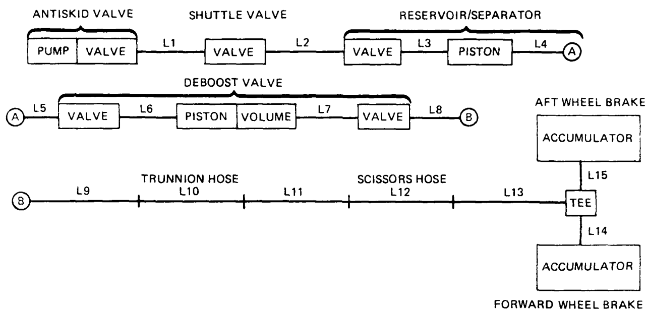
System Tube and Hose Data
