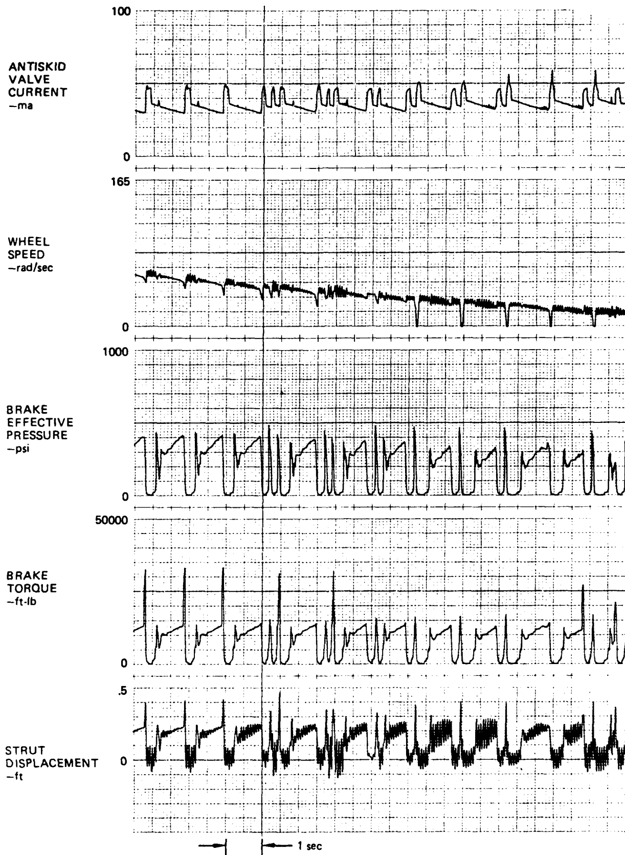
Figure 31. As-Built Brake System Stability at Room Temperature, Zero Strut Damping
