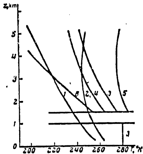
Figure 3.9 : Vertical temperature distribution for various models. [Ref. 10]
