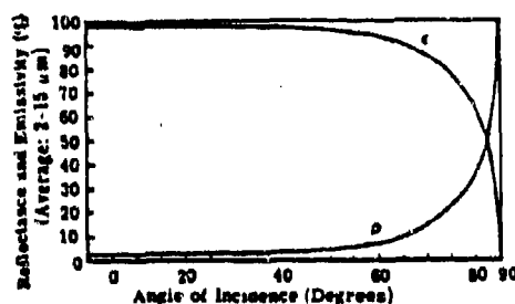
Figure 3.13 : Reflectance and emissivity of water ( 2 to 15 \mu\text{m} average ) versus angle of incidence. [Ref. 6]
