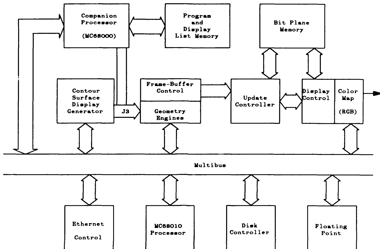
Figure 3 Block Diagram of the Silicon Graphics, Inc. IRIS (with additional, non-SGI Contour Surface Display Generator)
