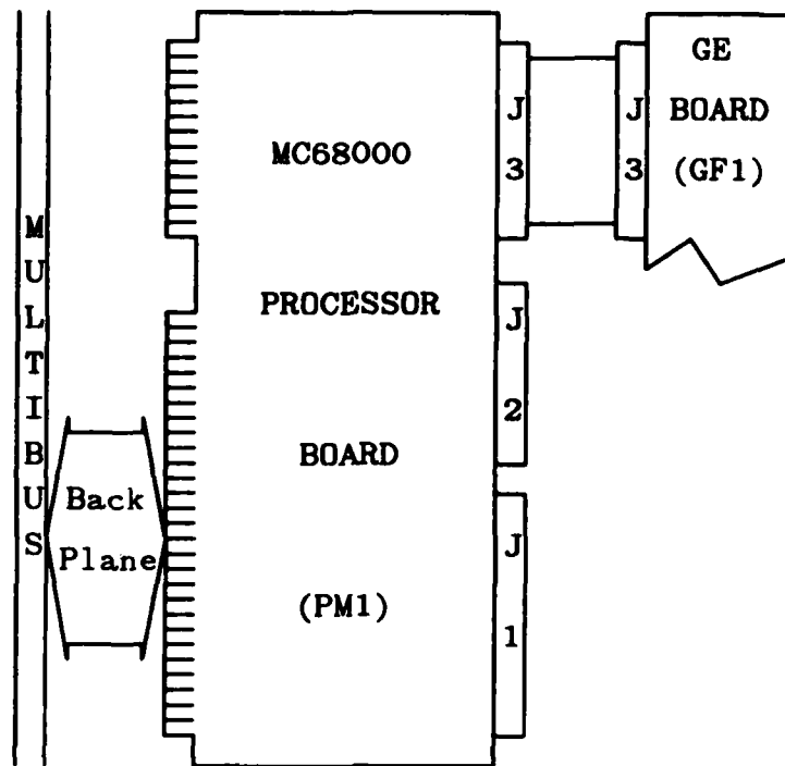
Figure 6a Silicon Graphics, Inc. IRIS Pipeline Connection for the Private Bus (Courtesy of Silicon Graphics, Inc.)
