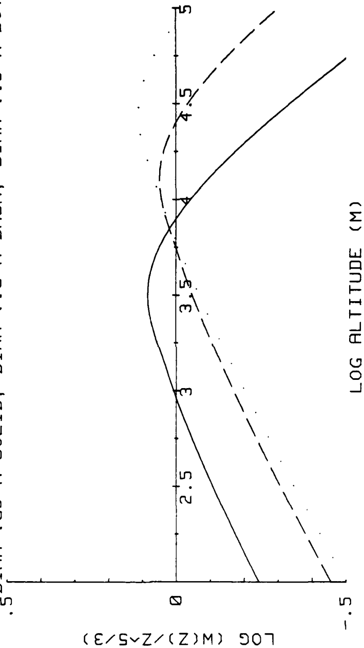
Figure 3.3 Error from z^{5/3} for Varying Top Hat Aperture Sizes
