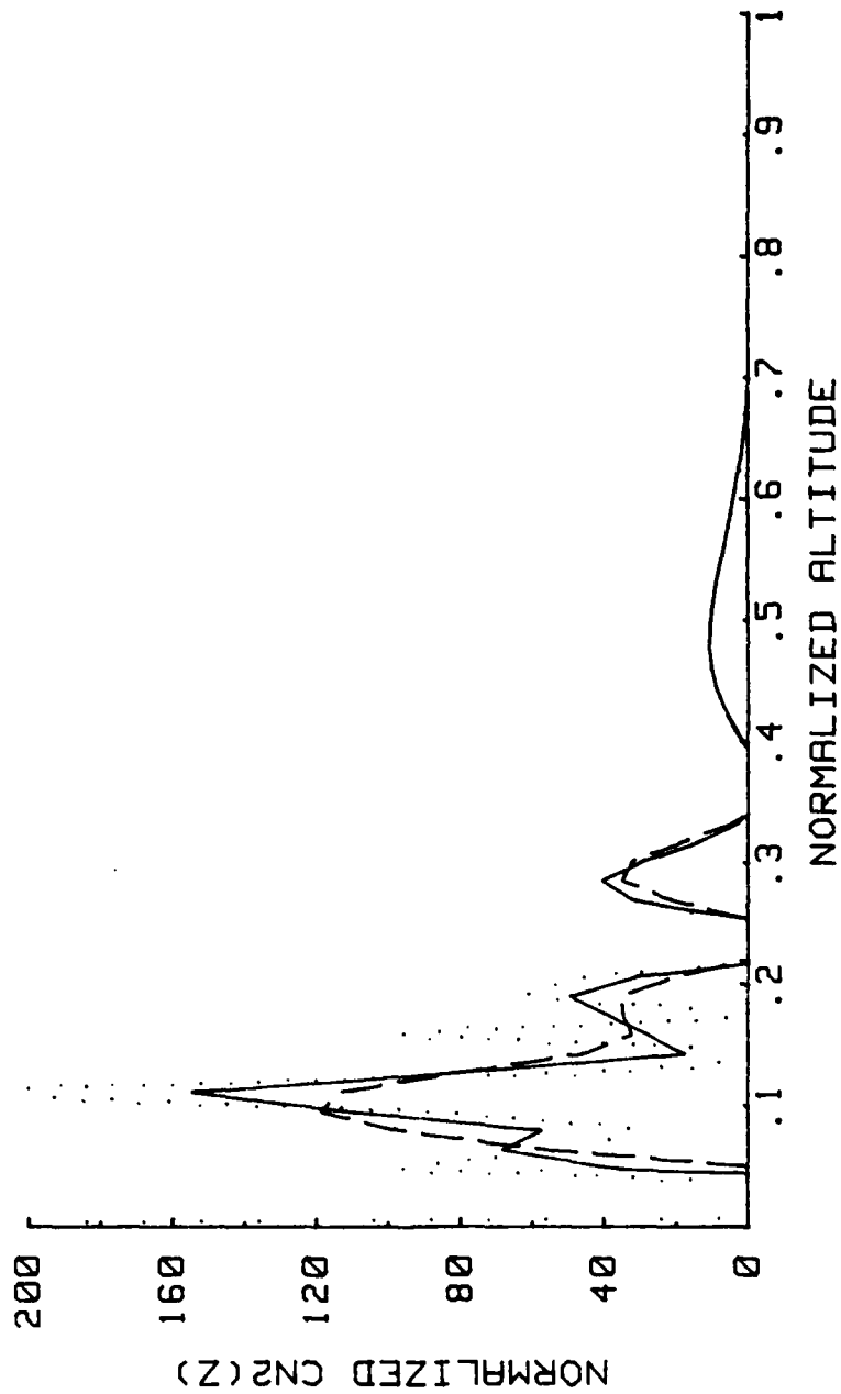
Figure 8.12 C_N^2(z) for Different Stabilizers
