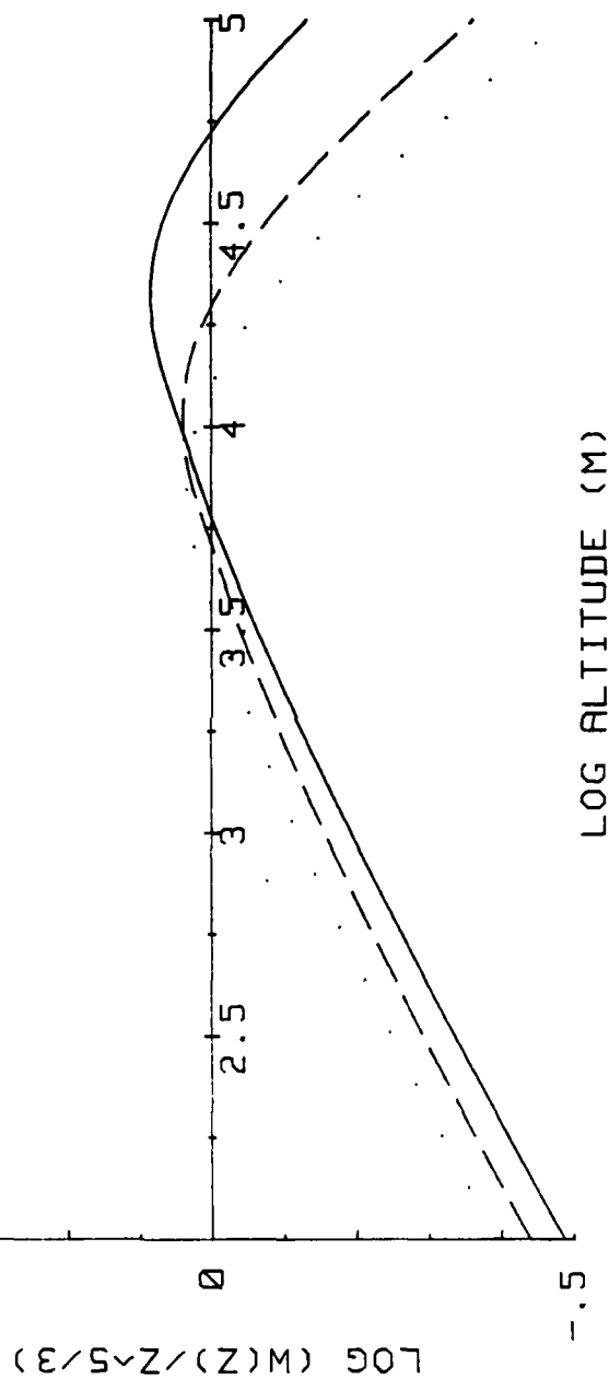
Figure 3.4 Wavelength Dependence of the Error from z^{5/3} for the Top Hat Aperture
