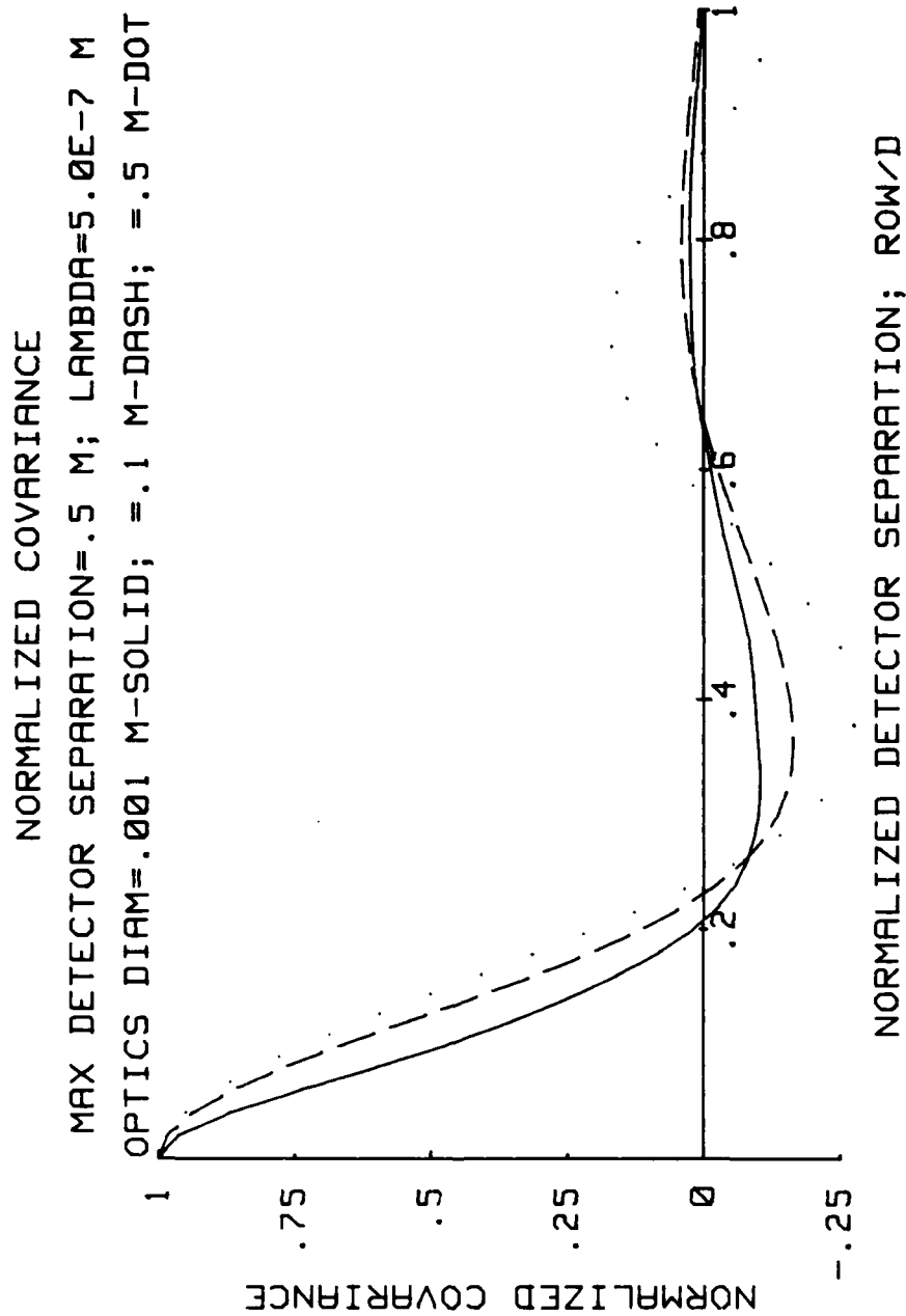
Figure 8.5 Covariance Function Dependence on Receiver Optics Aperture Size
