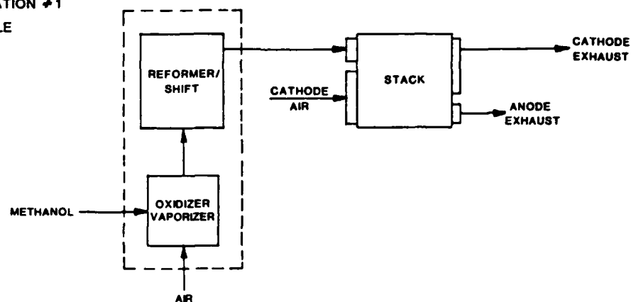
CONFIGURATION #2 CATHODE RECYCLE
