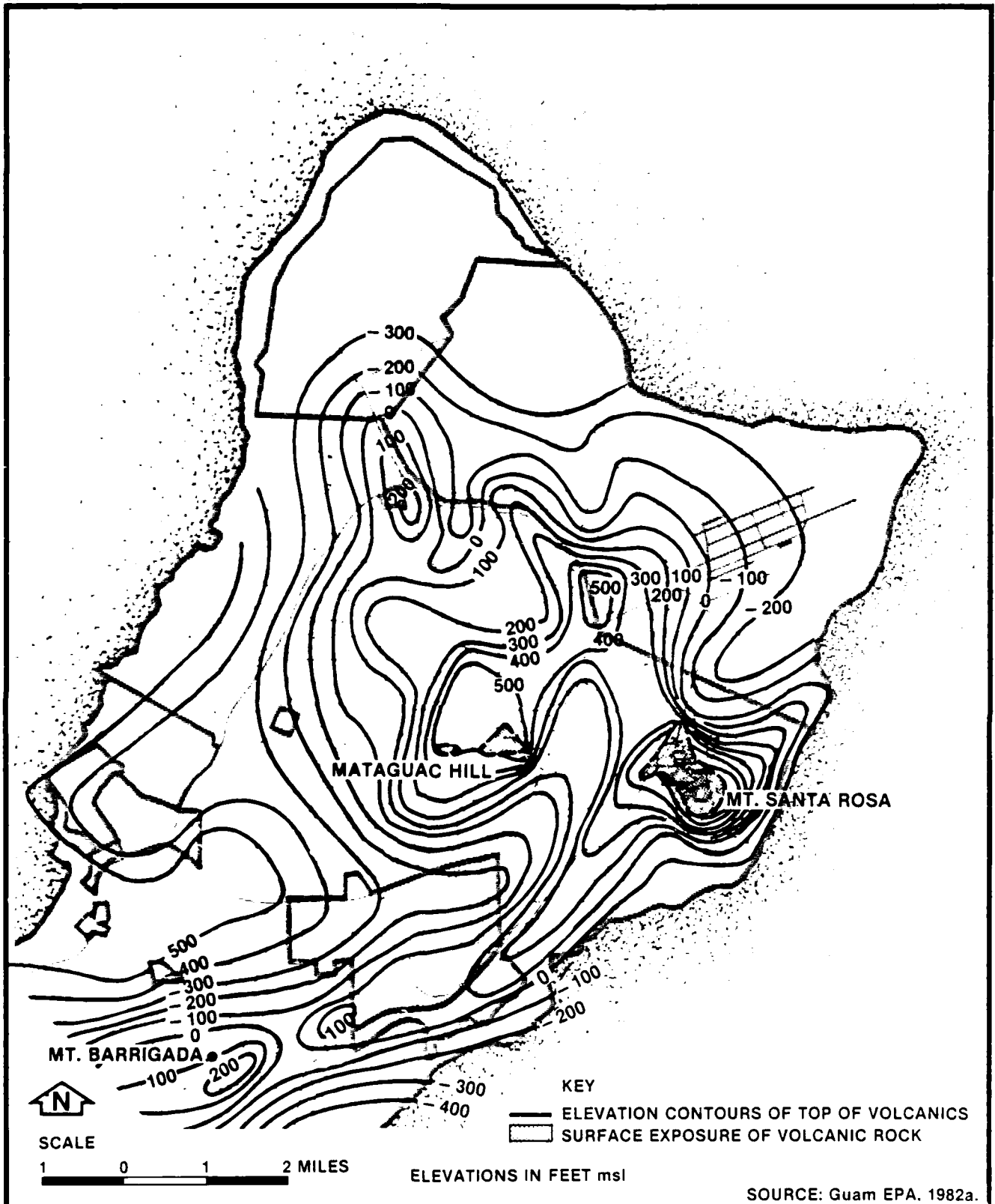
Figure 3.3-1 CONTOUR MAP OF THE VOLCANIC BASEMENT
