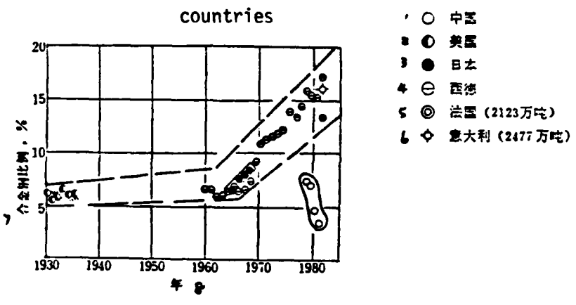
Figure 2 The percentane of alloy steel in overall production while annual capacity was between 30-40 million tons
