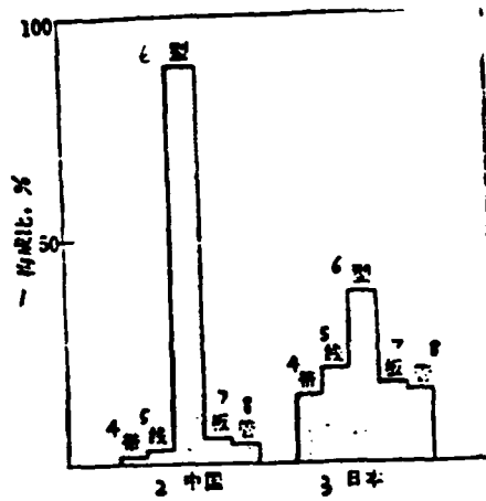
Figure 5 The comparison of compositions of special steel material in China and Japan for 1980
