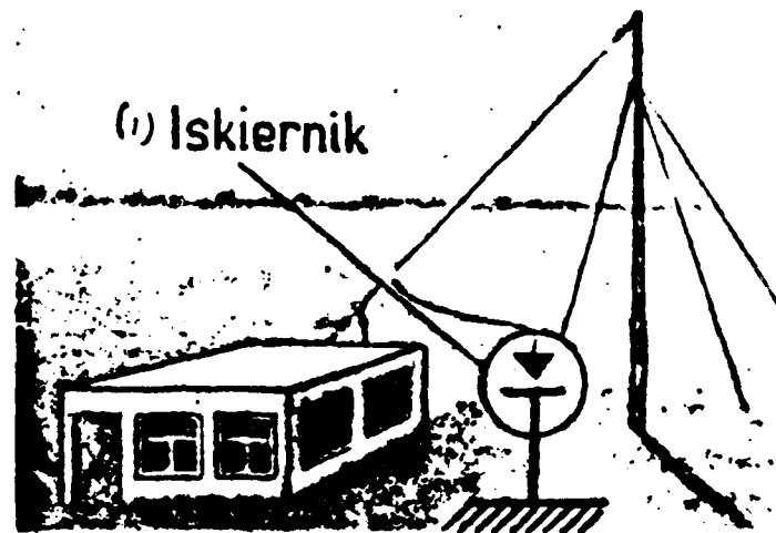
Picture 12. Protective spark gaps for safeguarding equipment connected to lines and antennas against overvoltage.
