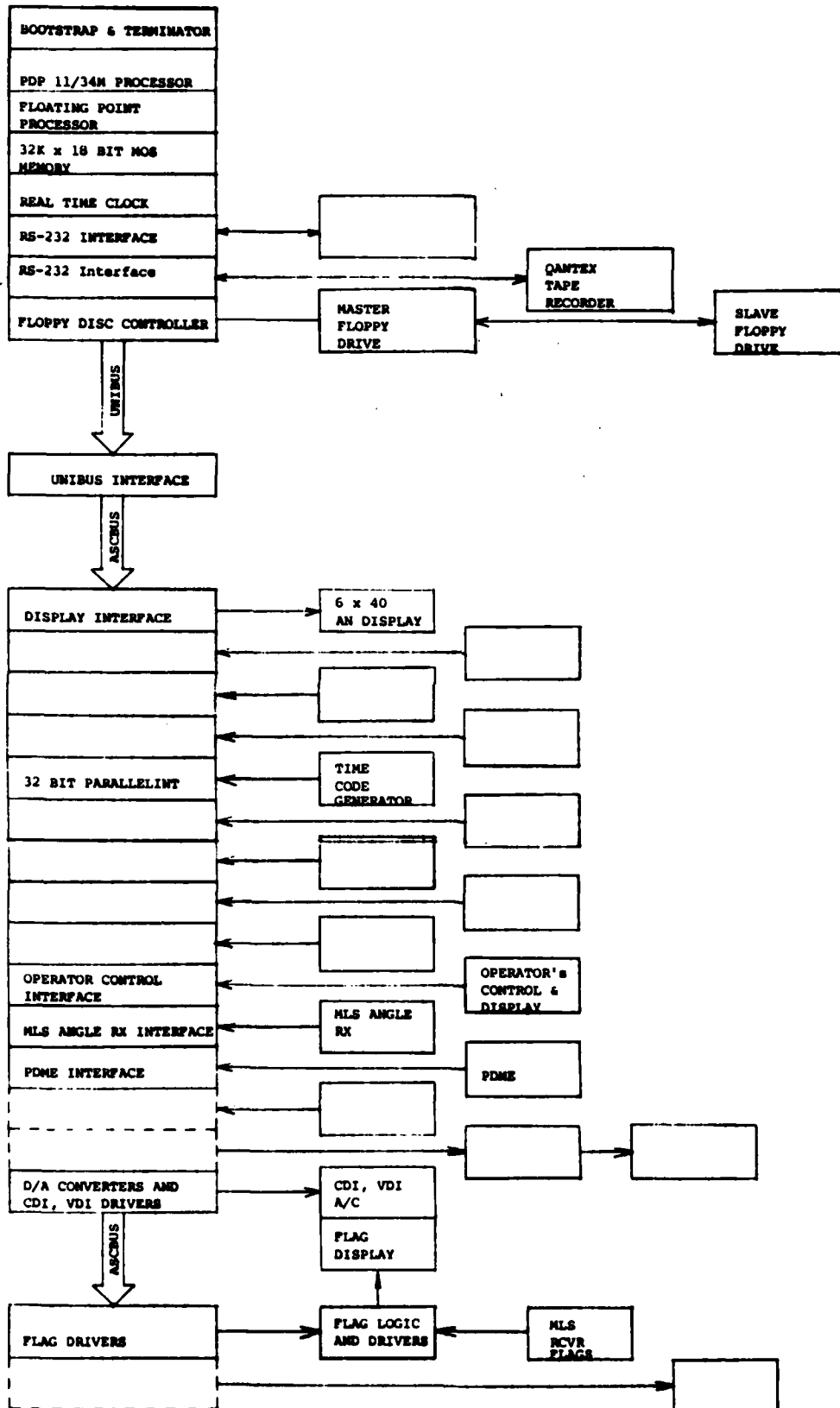
FIGURE 3. MLS COMPUTED CENTERLINE SYSTEM
