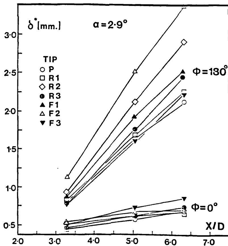
Figure 11. Wind and Leeside Development of \delta^* ( \alpha = 2.9^\circ )
