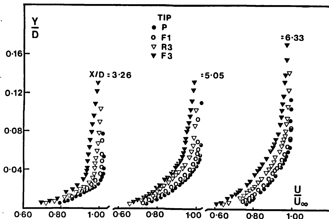
Figure 6. Boundary Layer Velocity Profile Development ( \alpha = 0^\circ )
