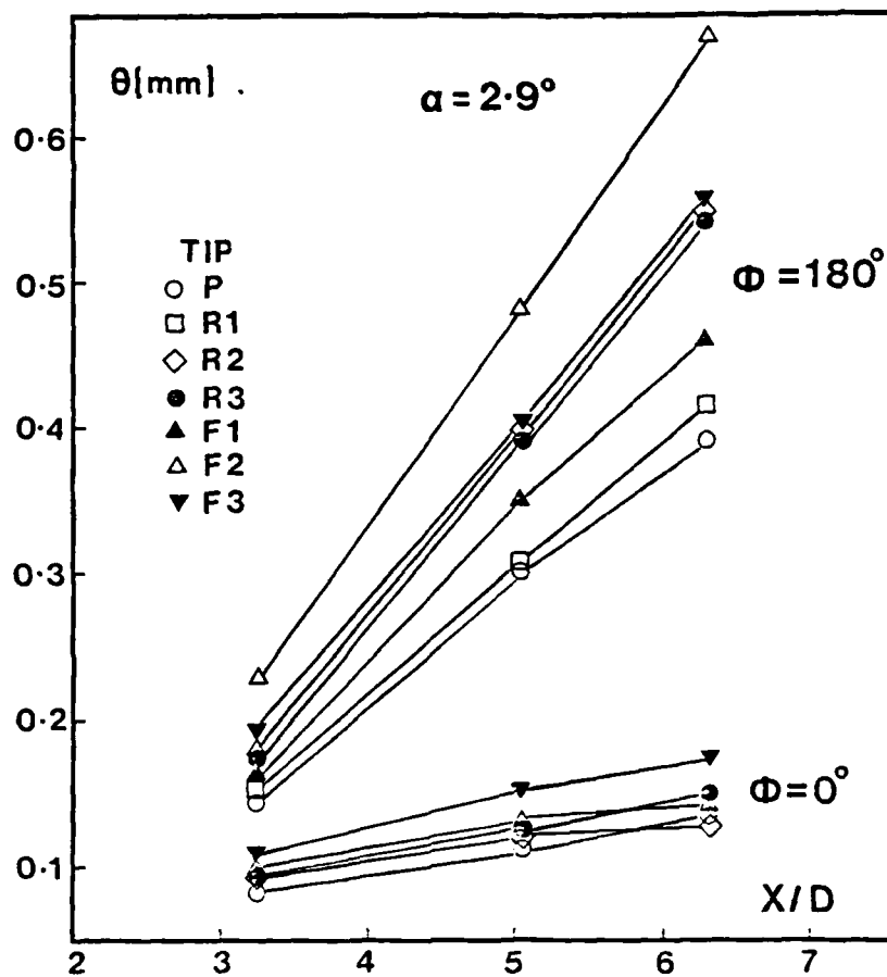
Figure 12. Wind and Leeward Development of \theta ( \alpha = 2.9^\circ )
