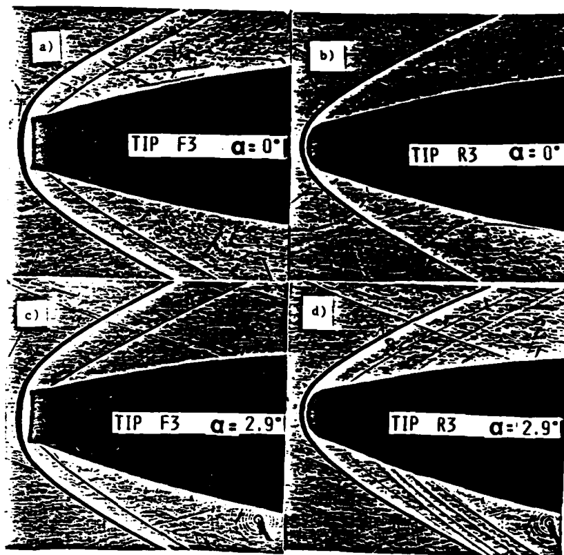
Figure 4. Shadow Photographs Using Tips R3 and F3
