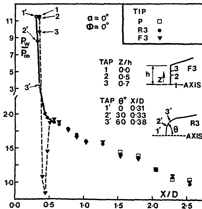
Figure 3. Pressure Distribution on the Ogive and Tip ( \alpha = 0^\circ )
