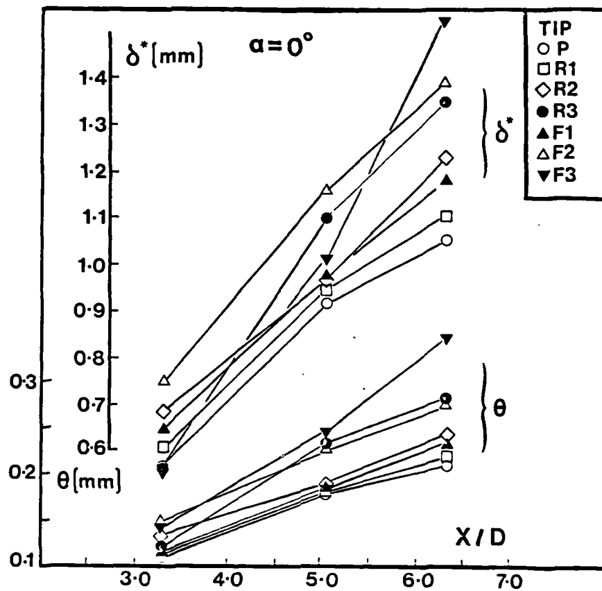
Figure 8. Streamwise Development of \delta^* and \theta ( \alpha = 0^\circ )
