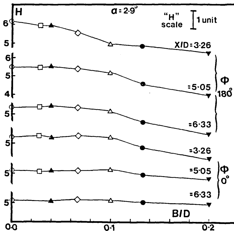
Figure 13. Boundary Layer Shape Factor as a Function of B/D ( \alpha = 2.9^\circ )
