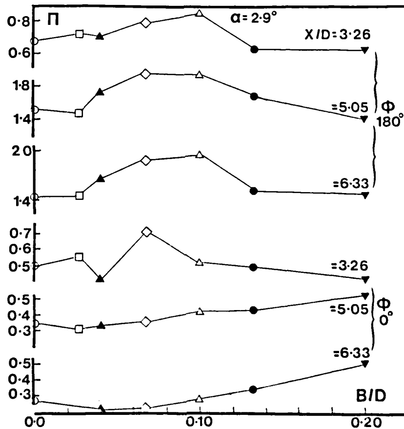
Figure 15. Wake Strength Parameter as a Function of B/D ( \alpha = 2.9^\circ )
