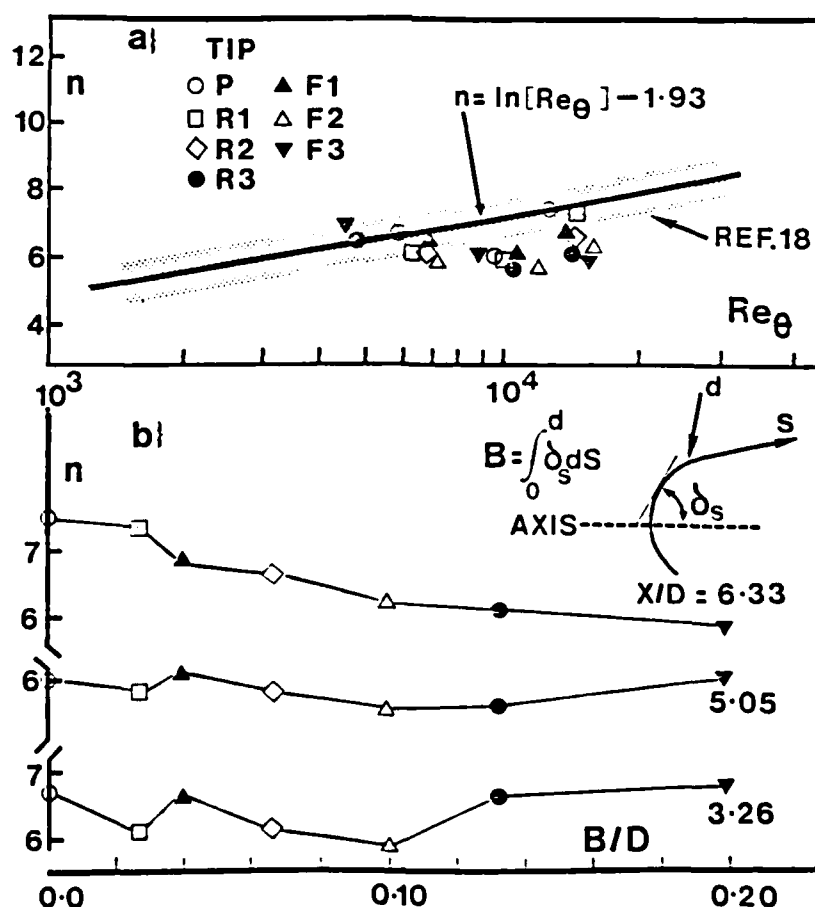
Figure 7. Boundary Layer Power Law Exponent n as a Function of Re_\theta and B/D
