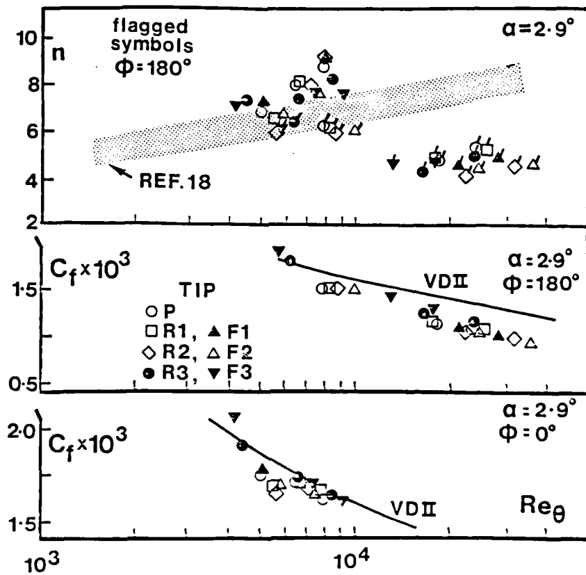
Figure 14. Velocity Profile Power Law Exponent and Skin Friction Coefficient as a Function of Re_\theta ( \alpha = 2.9^\circ )
