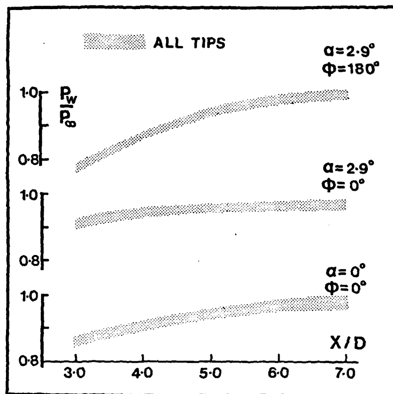
Figure 2. Pressure Distributions on Cylinder Body
