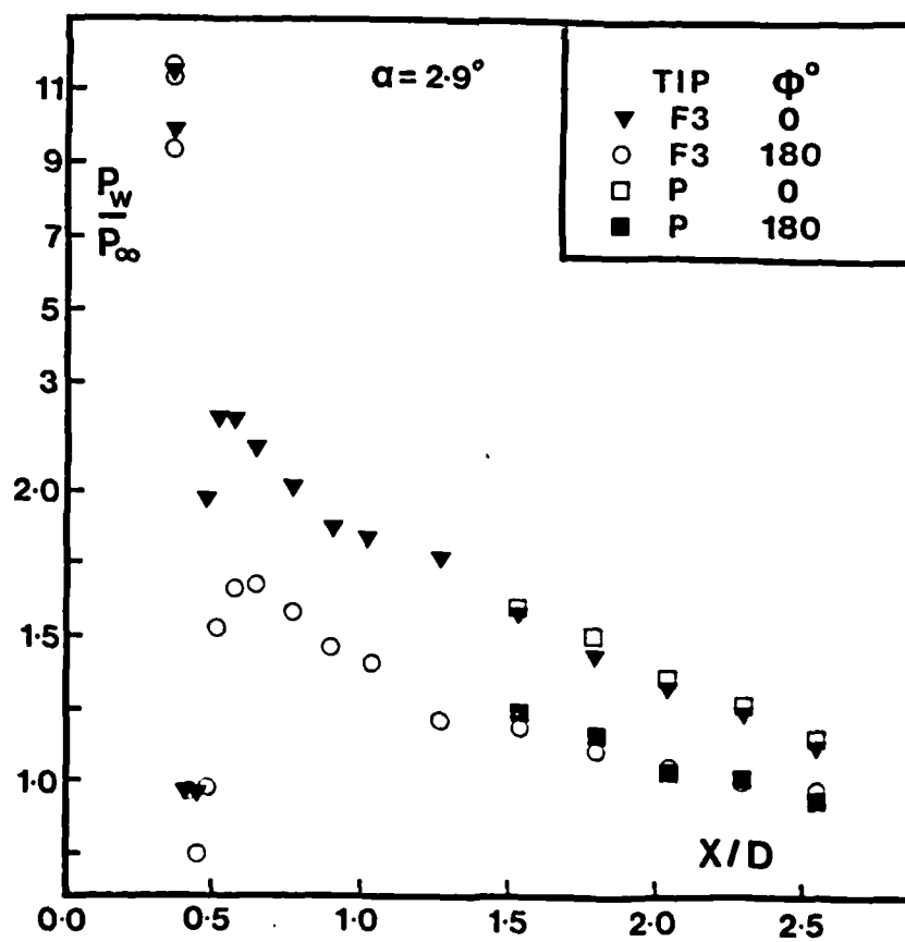
Figure 5. Pressure Distributions on the Ogive and Tip ( \alpha = 2.9^\circ )
