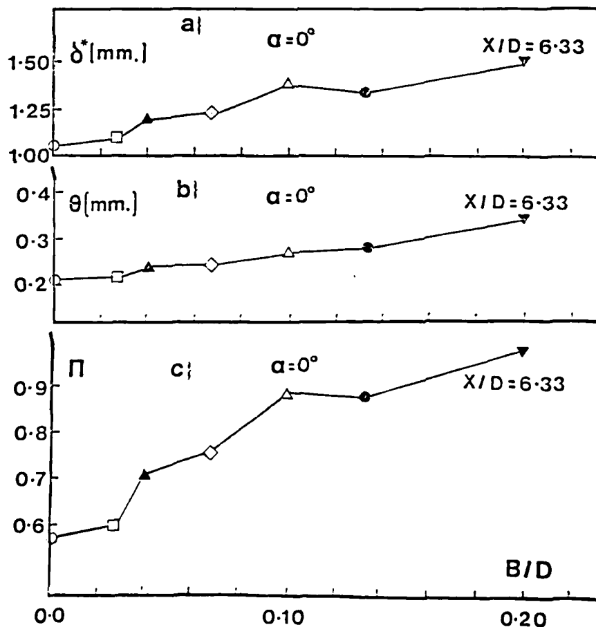
Figure 9. Correlation of, \delta^* , \theta and \Pi with B/D at Station 3 ( \alpha = 0^\circ )
