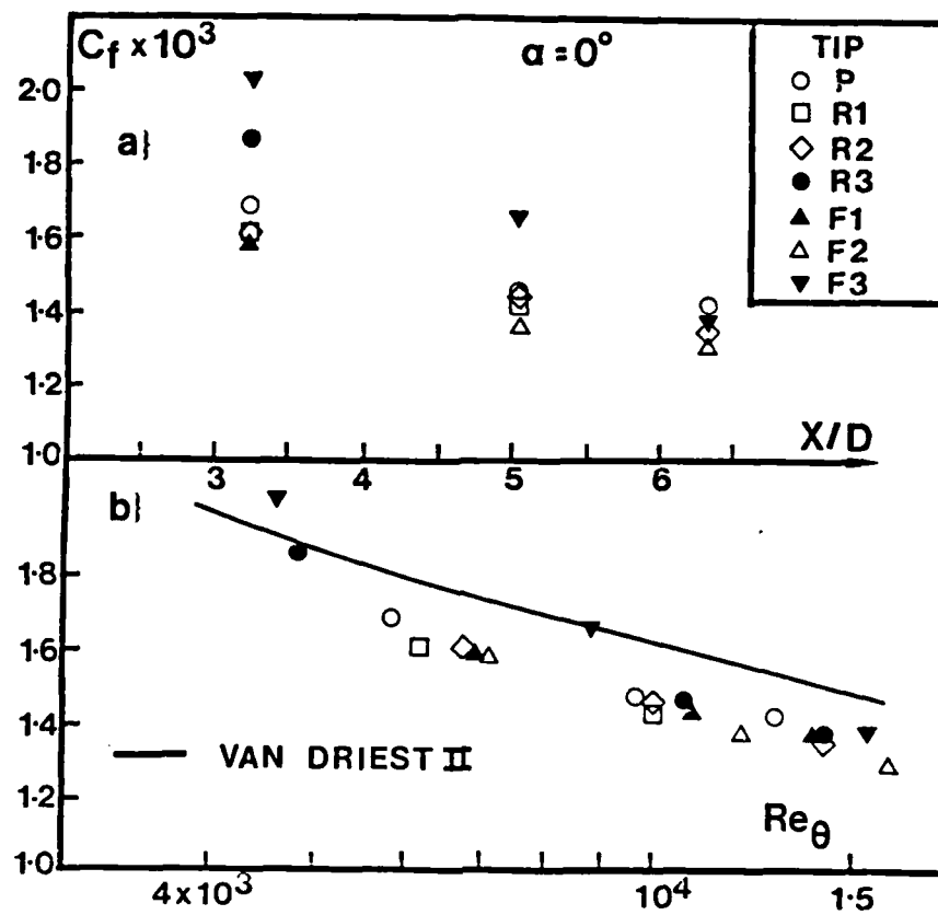
Figure 10. Skin Friction Coefficient as a Function of X/D and Re_\theta
