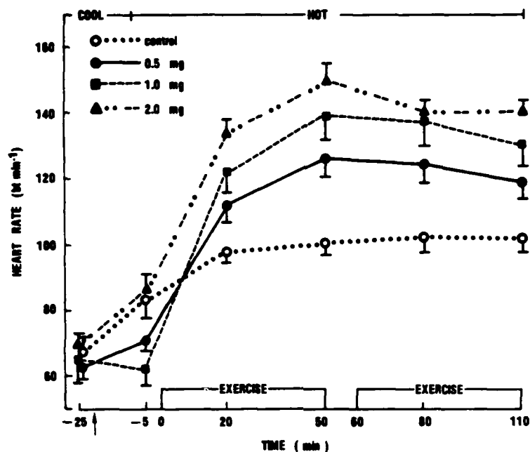
Figure 1. Heart rates ( \bar{X} \pm SE ) during rest in cool (20°C, 40% rh) and hot (40°C, 20% rh) environments and during two exercise bouts in the heat for control, 0.5, 1 and 2 mg atropine treatments. The arrow indicates the time of injection (n=7).
