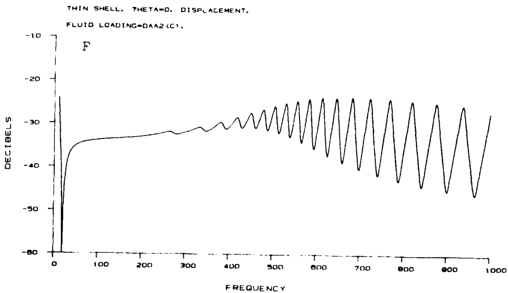
FIG.2 (cont.) DISPLACEMENT OF SHELL AT \theta=0
