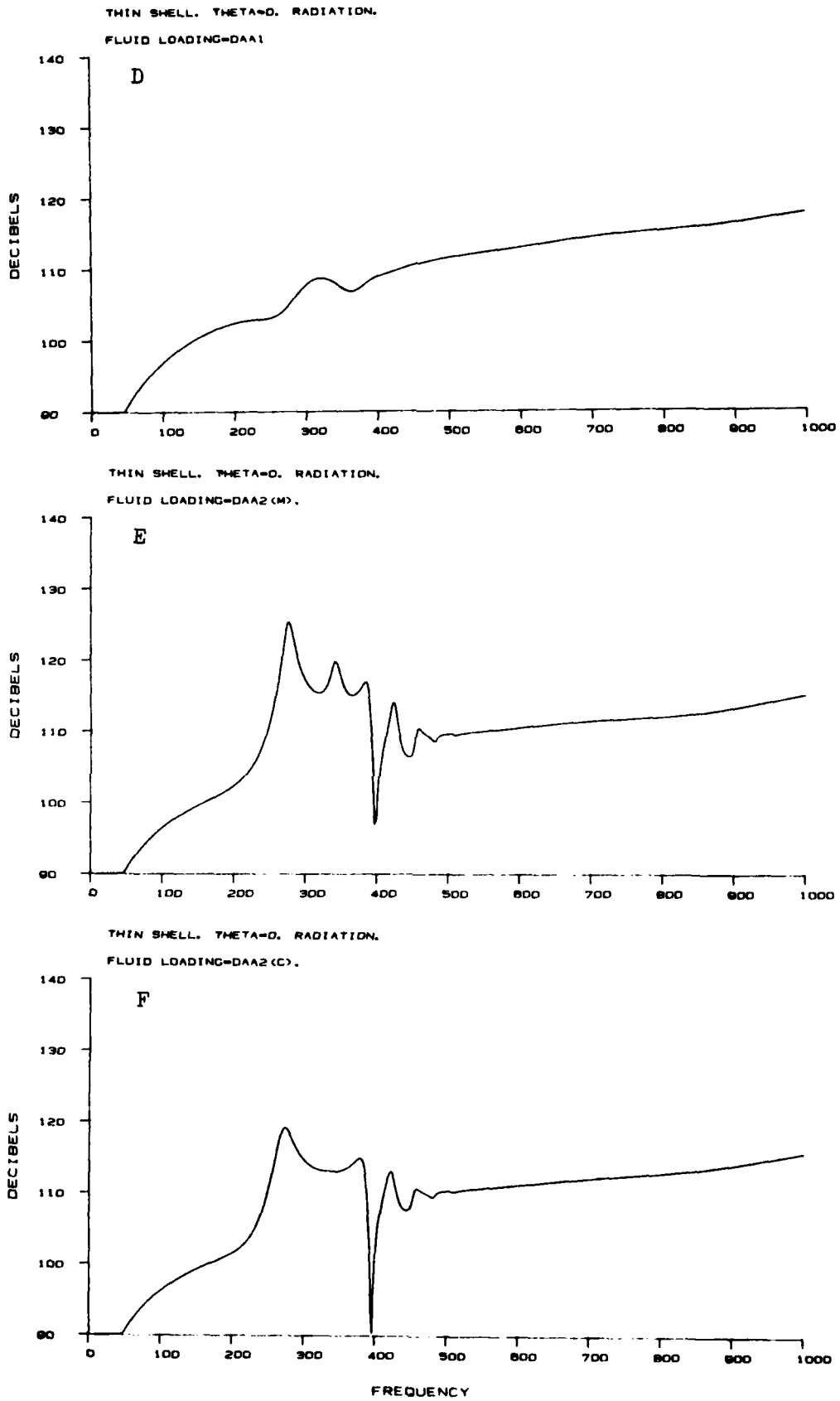
FIG.3 (cont.) SOUND RADIATION OF SHELL AT \theta=0
