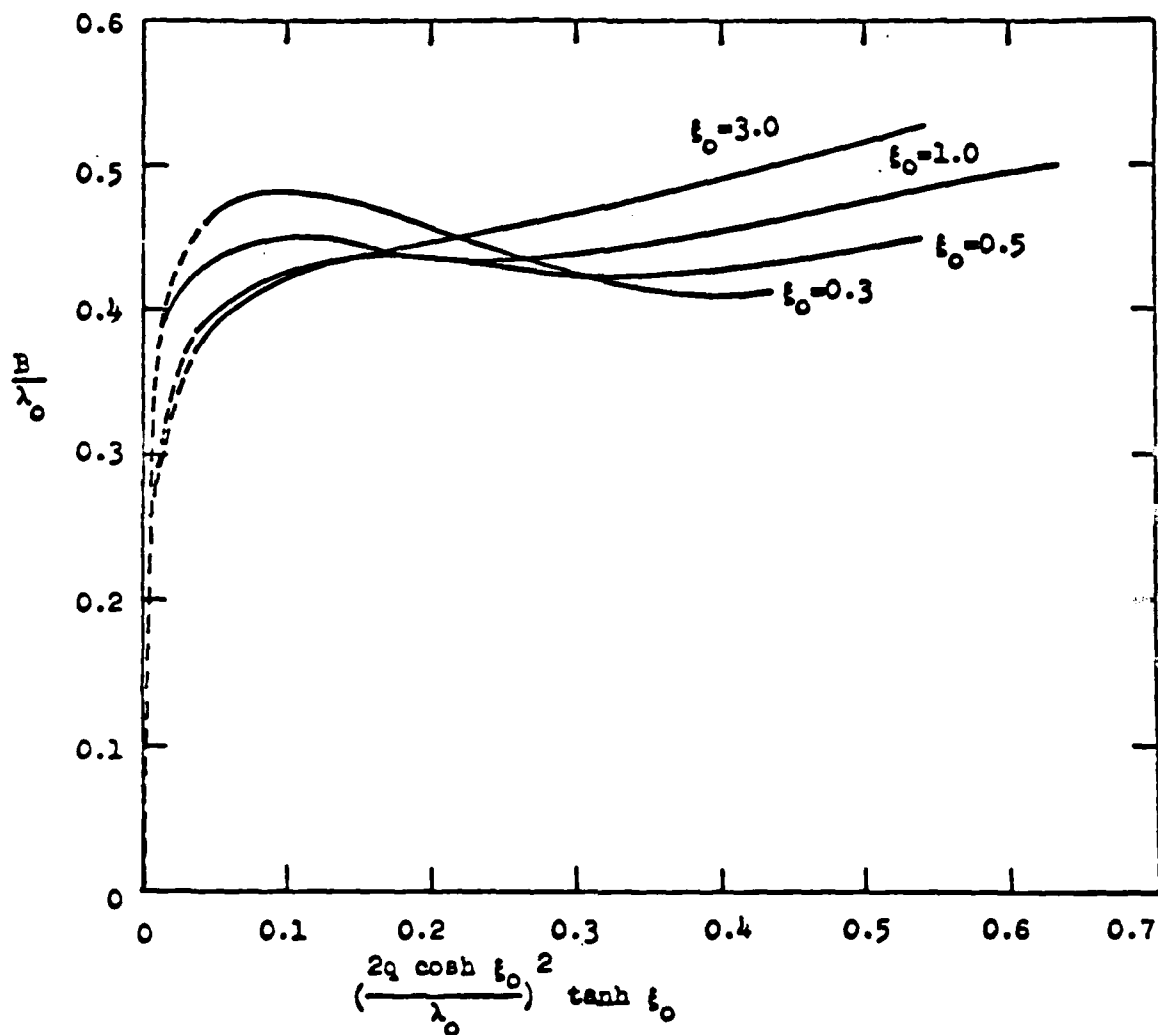
Fig. 2 Normalized axial electric field extent B/\lambda_0 as a function of normalized cross-sectional area for the HE_{11} mode. B is the distance measured from the origin to the point of observation where (E_x/E_{z_0})^2 = 0.1
