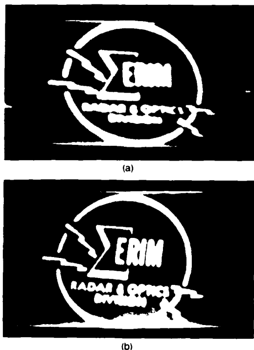
Fig. 3. Images of a transmissive object transmitted through a single fiber: (a) image of a transparency transmitted through a fiber with a 600- \mu\text{m} diam core; (b) image of a transparency transmitted through a fiber with a 200- \mu\text{m} diam core.
