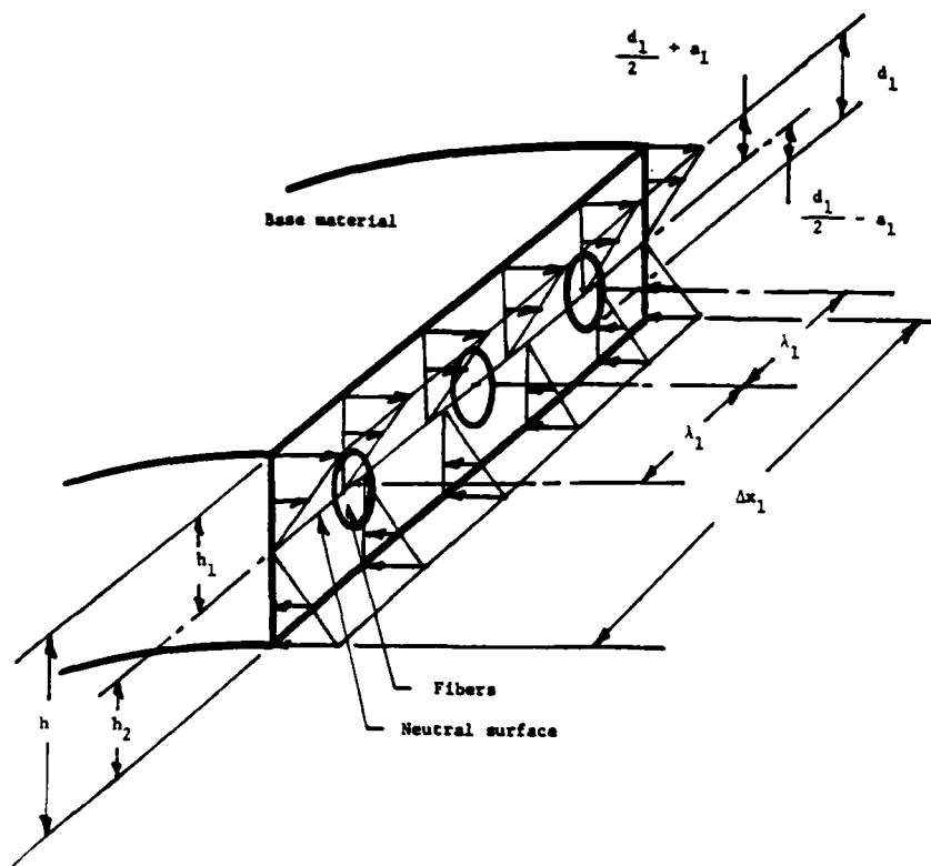
Figure 3.8 Schematic of a cross section indicating linear Kirchhoff type strain and middle surface location.
