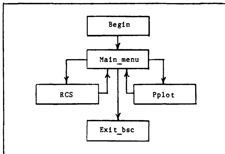
Fig. 18 Main Program
