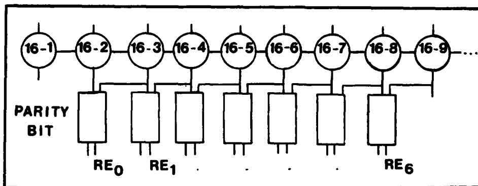
Figure 5.13 SIPO/XORSCAL Interface
