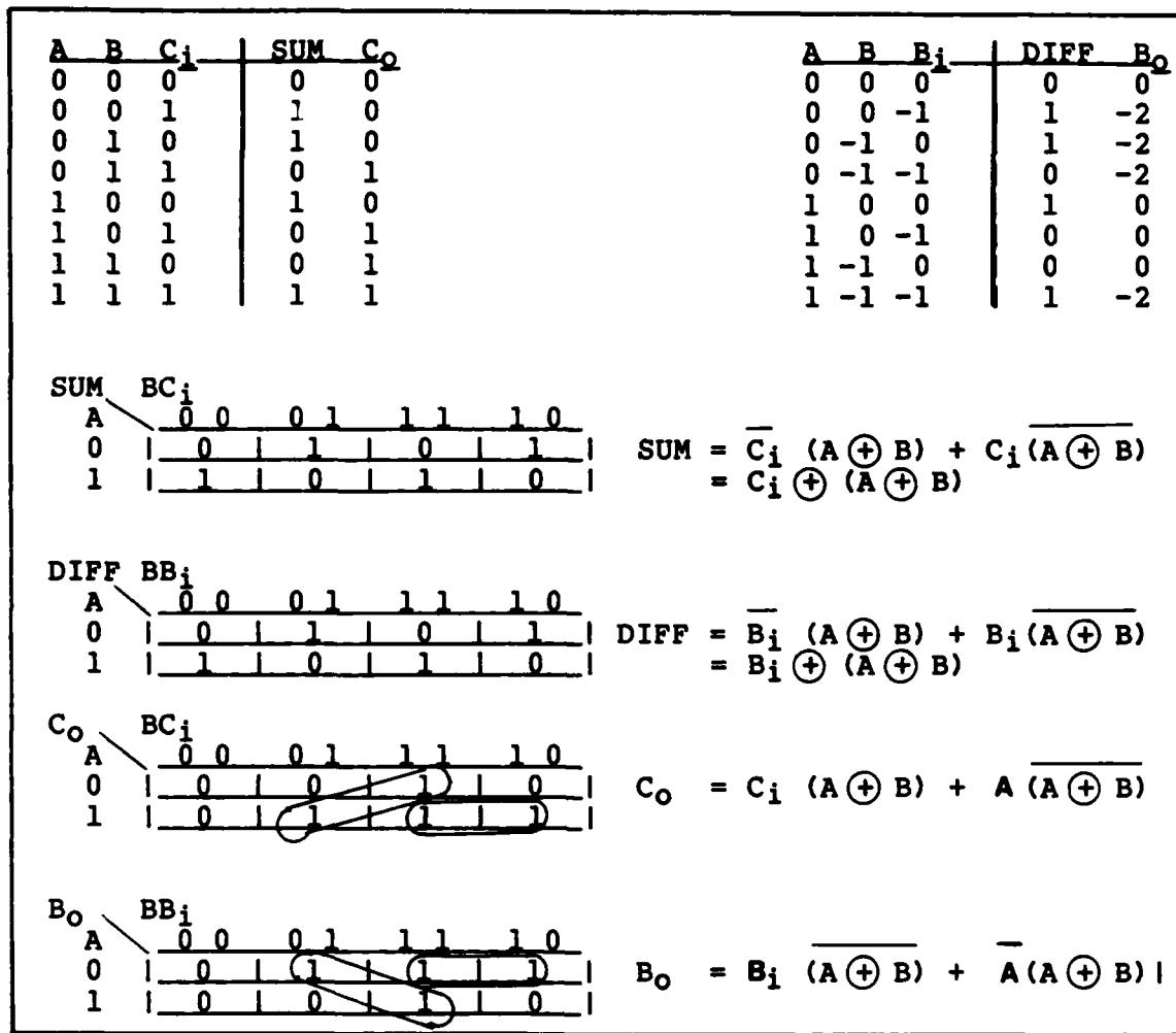
Figure 4.1 ADD/SUB Truth Tables and Boolean Equations
