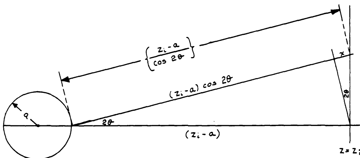
Fig. 3.2. Analysis of Telescope Alignment Error
