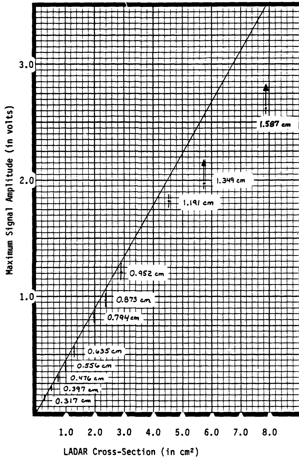
Fig. 5.3. Comparison of Predicted and Measured LRCS Values for the Spherical Standards (each data point annotated with its relevant sphere's radius)
