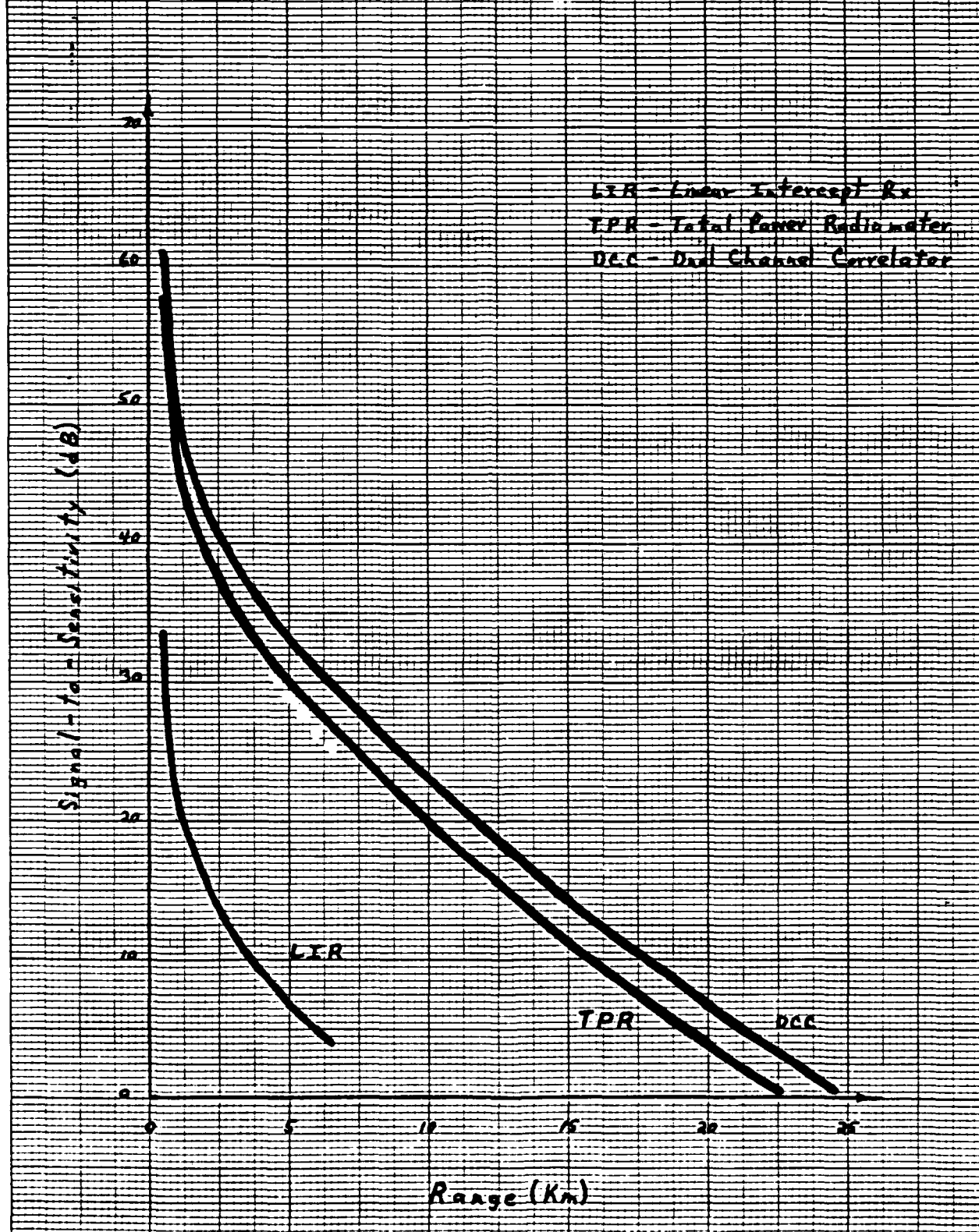
Figure 3.14 Comparison of the Performance of Interceptors
