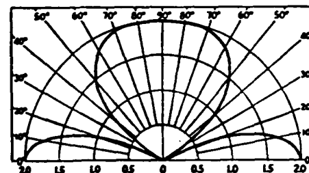
Vertical dipole antenna with center 1/2 wavelength high.
