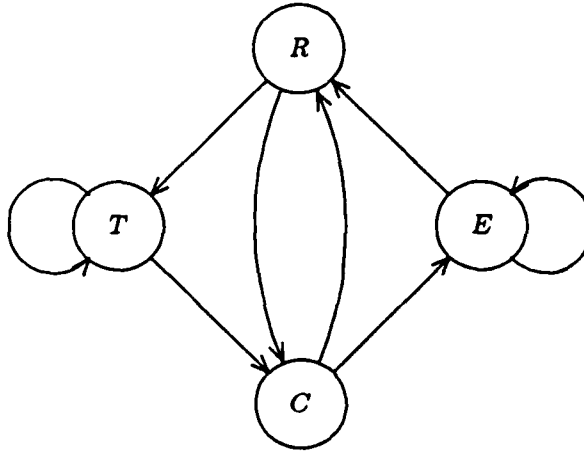
Figure 8: Possible region changes.
