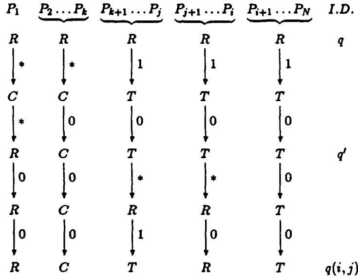
Figure 10: The Lower Bound Construction.
