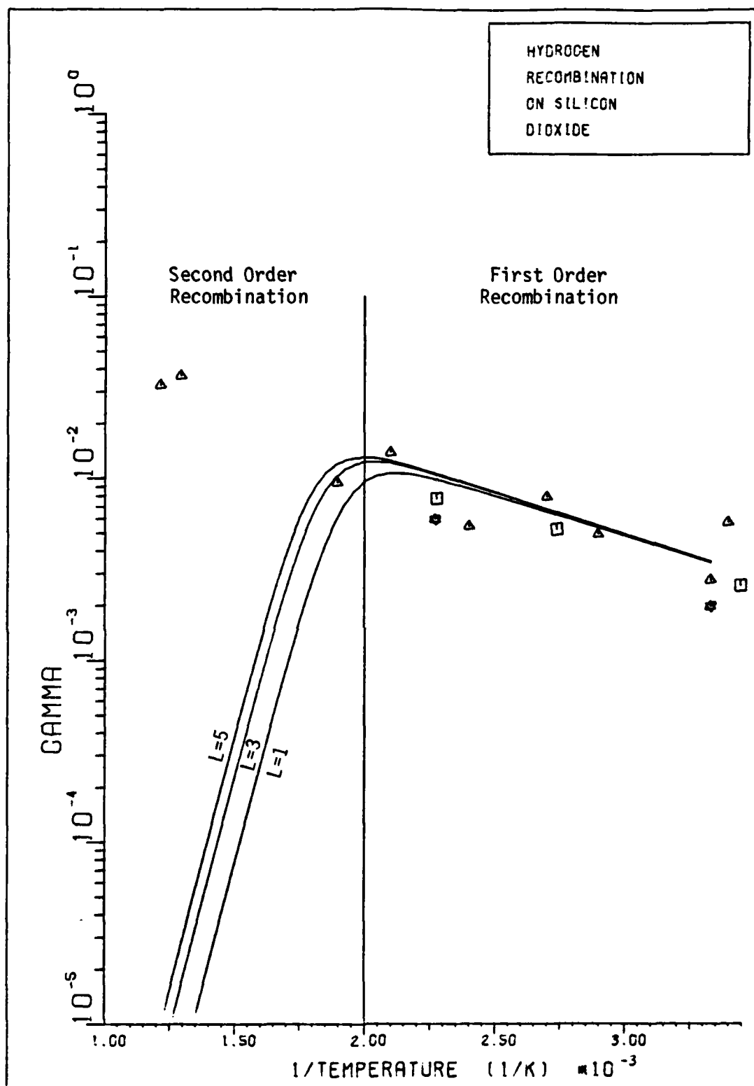
Figure 21. Hydrogen Recombination Coefficient vs. 1/\text{Temperature} for S_0 = 0.15 L \exp(-0.002 T) for L = 1, 3, 5 .
