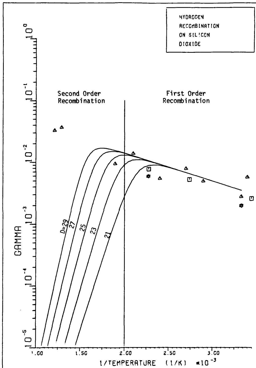
Figure 22. Hydrogen Recombination Coefficient vs. 1/\text{Temperature} for Bond Energy, D = 21, 23, 25, 27, 29 kcal/mole.
