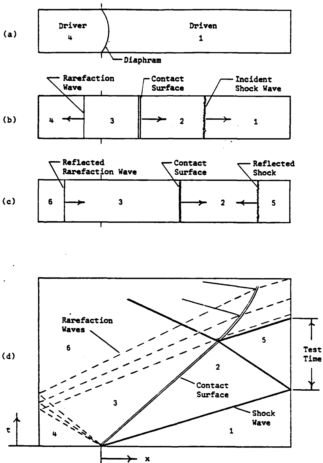
Figure 1: Shock Tube Wave Phenomena
