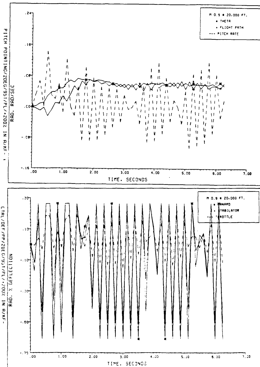
Fig. F.6. Aircraft Response with Actuators, Position Limits, and Kalman Filter in the Loop/Control Based on \bar{x}(t_i)/200 Percent increase in F Matrix a. Aircraft responses; b. Control deflections
