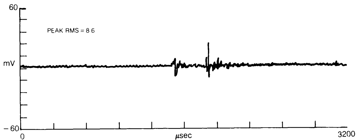
A) TRANSDUCER C OUTPUT (FILTERED)
