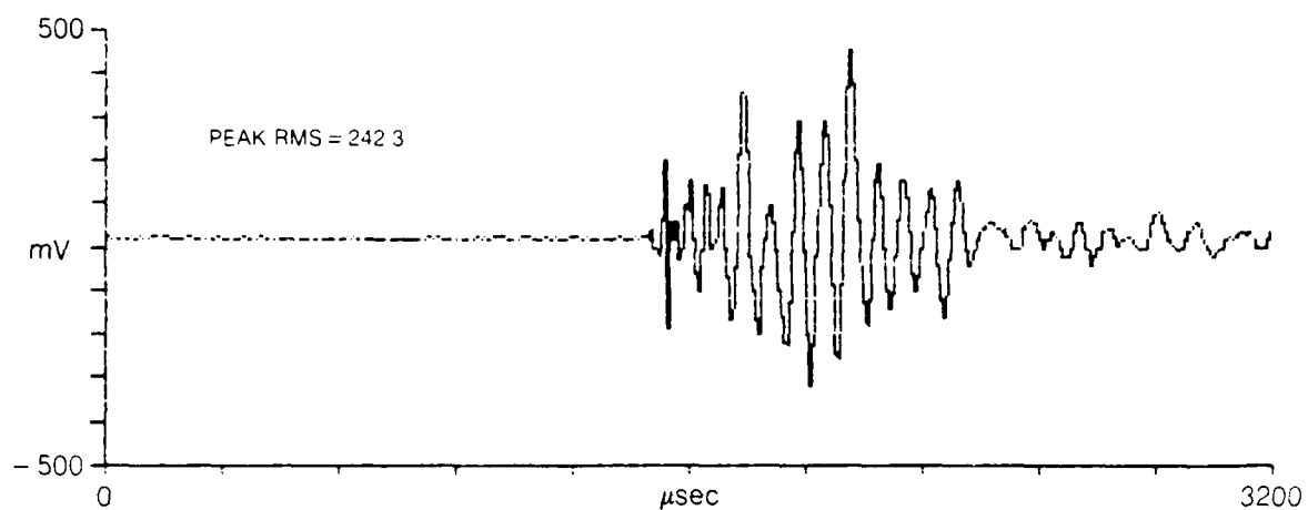
A) TRANSDUCER A OUTPUT
