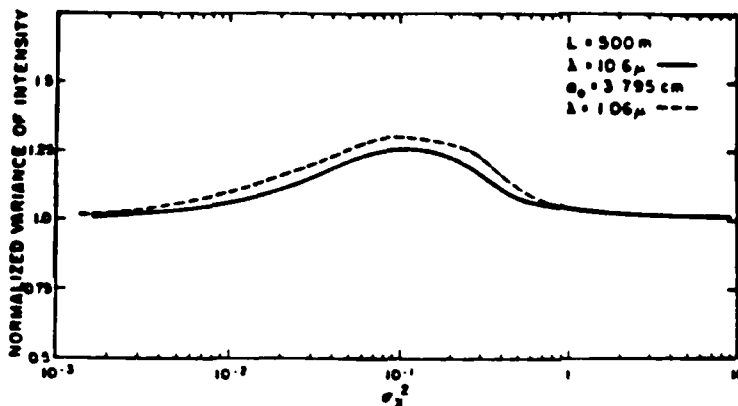
Figure 3. Normalized variance of the received intensity versus the log-amplitude variance, focused beam, 500-m range, 1.06- and 10.6- \mu m wavelengths, \sigma_0 = 3.795 cm.
