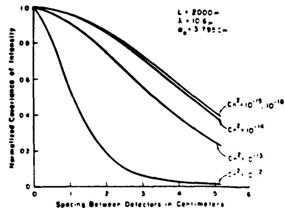
Figure 4. Normalized covariance of the received intensity, focused beam, 2000-m range, 10.6- \mu m wavelength, \sigma_0 = 3.795 cm.
