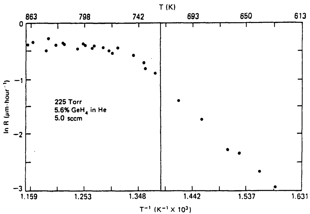
Figure 4. Arrhenius Plot Showing Laser Initiated Chemical Vapor Deposition Below 718 K.
