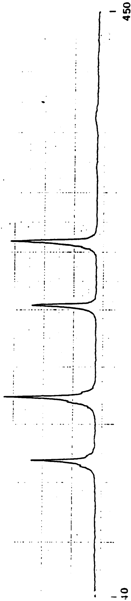
Figure 1. (top) MPI spectrum of TMA in the blue (after reference 1) and (bottom) expanded view of the region between 440 nm and 450 nm (acquired in our laboratory).
